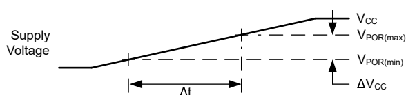
Figure 6-6. Voltage Waveforms, Supply Ramp
