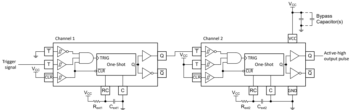
Figure 8-4. Delayed Pulse Generation Schematic Using the TPUL2G223-Q1
