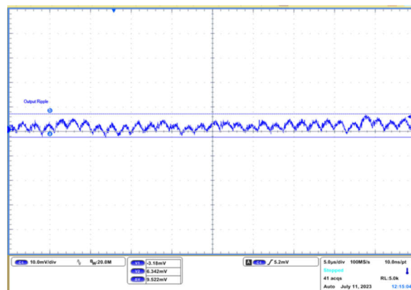
Figure 9-18. V_{OUT} Steady-State Ripple
