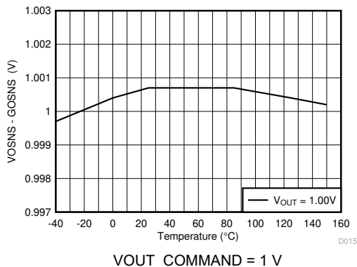
Figure 7-5. Output Voltage vs Junction Temperature
