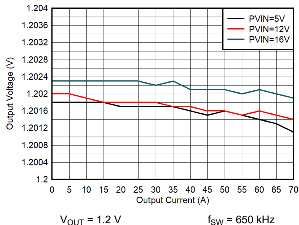
Figure 9-12. Load Regulation
