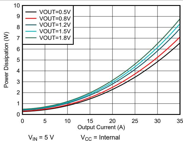
Figure 7-3. TPSM8S6C24 Power Dissipation vs Output Current
