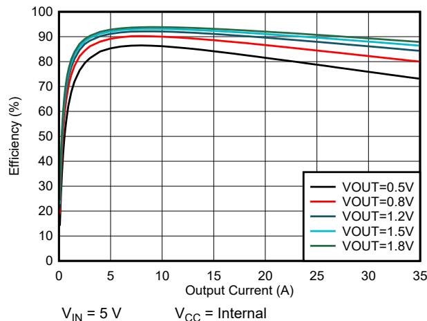
Figure 7-1. TPSM8S6C24 Efficiency vs Output Current
