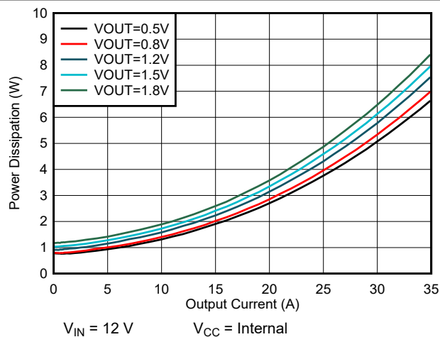
Figure 7-4. TPSM8S6C24 Power Dissipation vs Output Current
