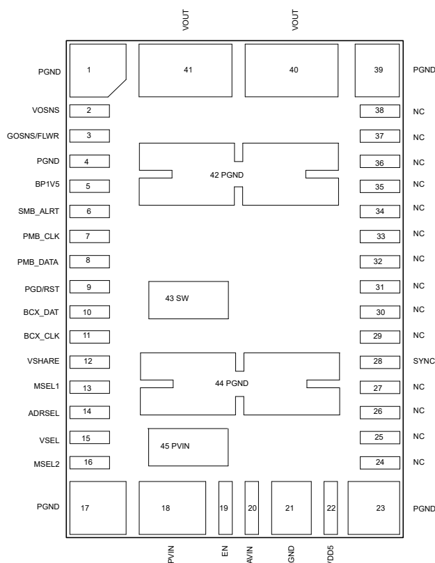
Figure 6-1. 45-Pin QFM-MOY Package (Top View)
