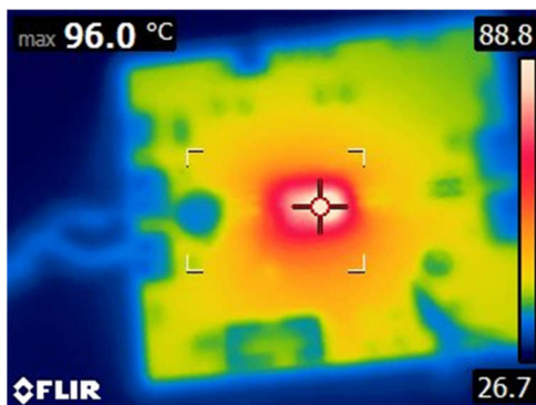
Figure 9-24. Thermal Image at 25^\circ\text{C} Ambient, 12 Vin, 1.2V, 35 A, 650 kHz
