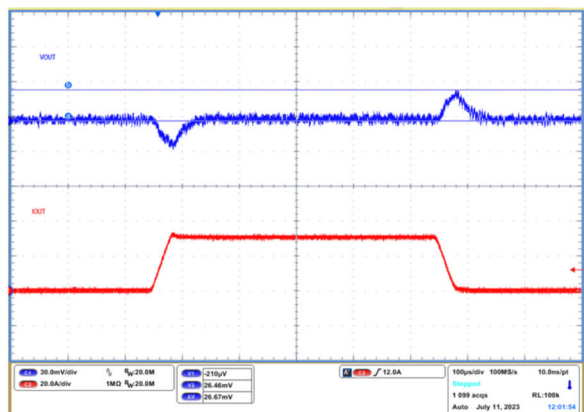
Figure 9-17. Load Transient Response
