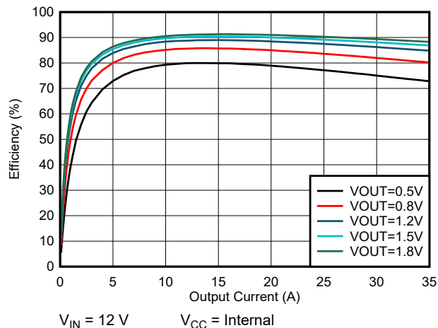
Figure 7-2. TPSM8S6C24 Efficiency vs Output Current
