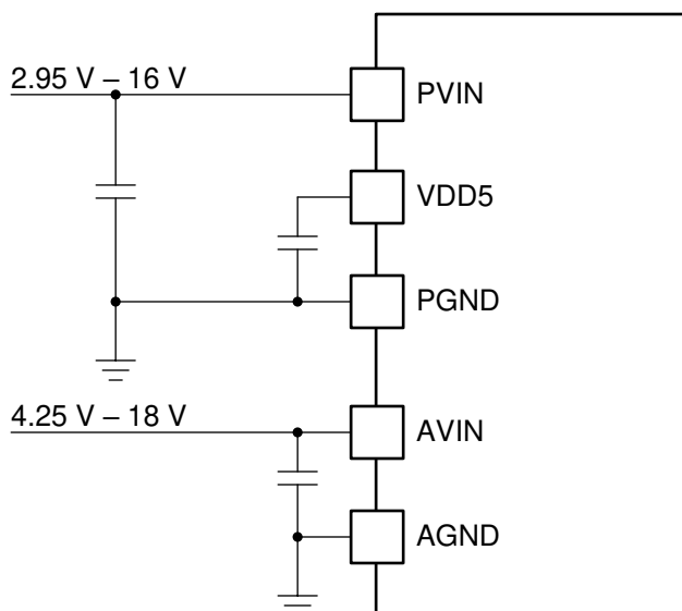
Figure 8-2. TPSM8S6C24 Separate PVIN and AVIN Connections
