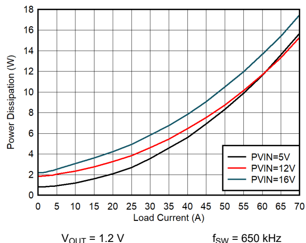
Figure 9-14. Power Dissipation
