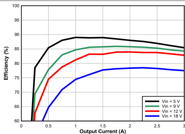
Figure 7-4. Efficiency
