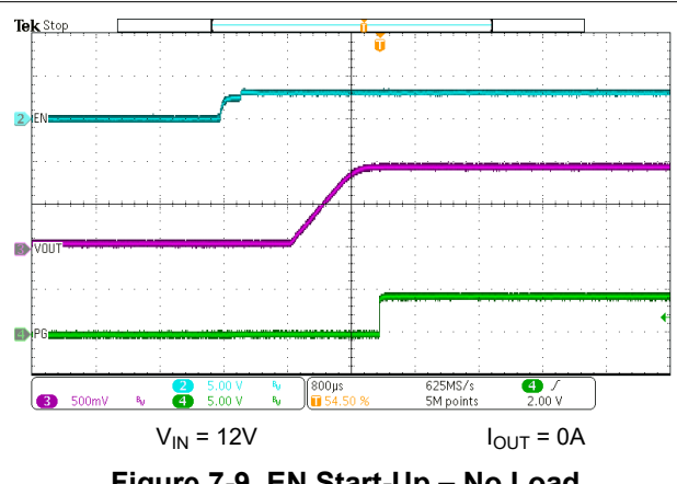
Figure 7-9. EN Start-Up – No Load
