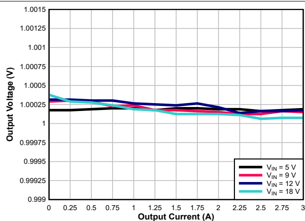
Figure 7-5. Load Regulation
