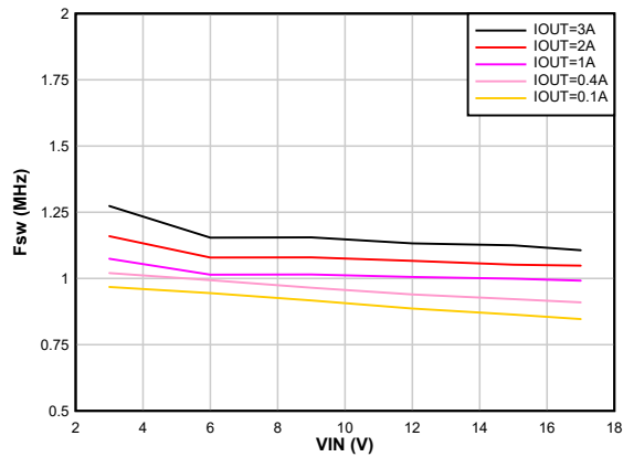
Figure 8-17. Switching Frequency vs Input Voltage V_{OUT} = 1.2 \text{ V}
