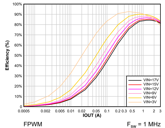
Figure 8-10. Efficiency vs Output Current V_{OUT} = 1.8 \text{ V}
