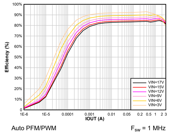
Figure 8-8. Efficiency vs Output Current V_{OUT} = 1.8 \text{ V}
