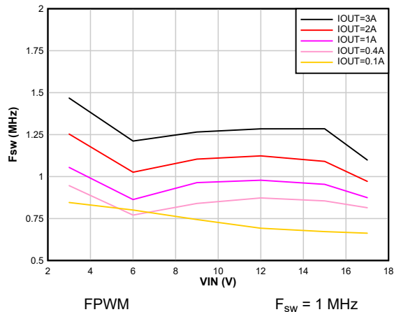
FPWM F_{sw} = 1 \text{ MHz} Figure 8-58. Switching Frequency vs Input Voltage V_{OUT} = 0.4 \text{ V}
