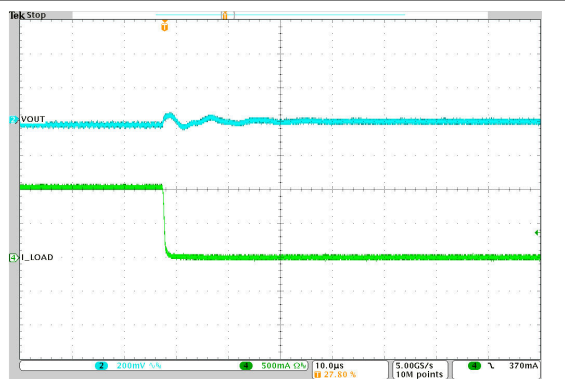
V_{IN} = 12\text{ V} 1-MHz Auto PFM/PWM I_O = 1\text{ A to }5\text{ mA} V_{OUT} = 1.2\text{ V} T_A = 25^\circ\text{C}
