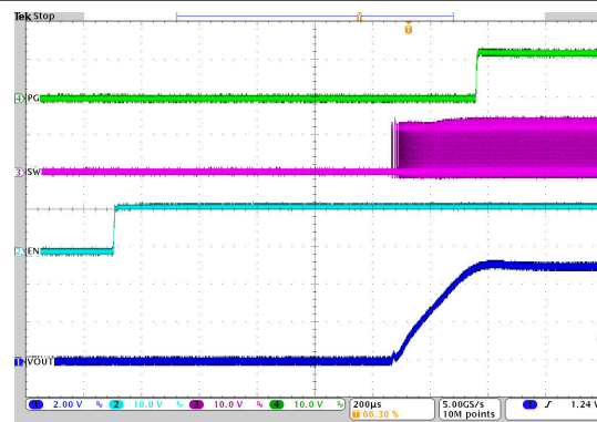
Figure 8-26. Start-Up Timing
