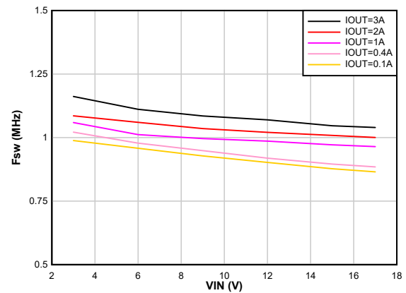
Figure 8-18. Switching Frequency vs Input Voltage V_{OUT} = 1.8 \text{ V}
