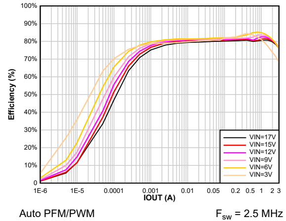
Figure 8-6. Efficiency vs Output Current V_{OUT} = 1.2 \text{ V}
