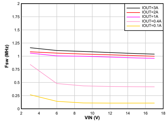
Figure 8-18. Switching Frequency vs Input Voltage V_{OUT} = 1.8 \text{ V}
