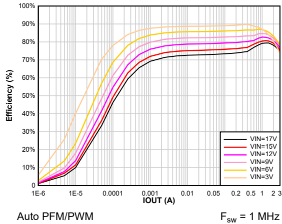
Figure 8-5. Efficiency vs Output Current V_{OUT} = 1.2 \text{ V}
