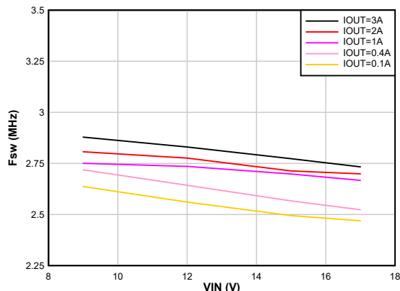
Figure 8-24. Switching Frequency vs Input Voltage V_{OUT} = 5.5 \text{ V}
