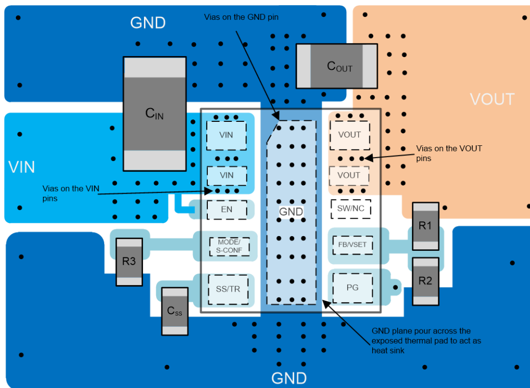
Figure 8-61. Layout
