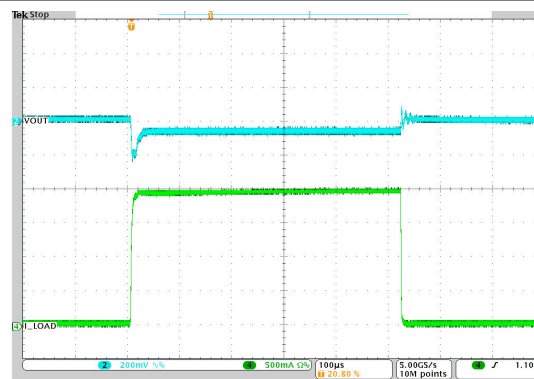
V_{IN} = 12\text{ V} I_O = 5\text{ mA to }2\text{ A to }5\text{ mA} V_{OUT} = 3.3\text{ V} 2.5-MHz Auto PFM/PWM T_A = 25^\circ\text{C}
