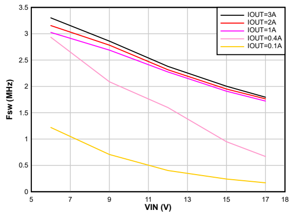
Figure 8-19. Switching Frequency vs Input Voltage V_{OUT} = 1.8 \text{ V}
