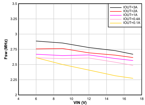
Figure 8-20. Switching Frequency vs Input Voltage V_{OUT} = 1.8 \text{ V}
