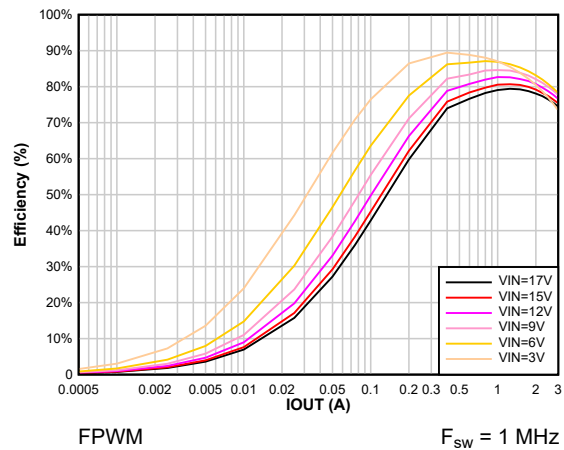
Figure 8-7. Efficiency vs Output Current V_{OUT} = 1.2 \text{ V}
