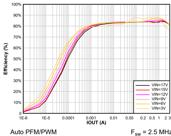
Figure 8-9. Efficiency vs Output Current V_{OUT} = 1.8 \text{ V}
