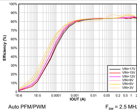
Figure 8-9. Efficiency vs Output Current V_{OUT} = 1.8 \text{ V}
