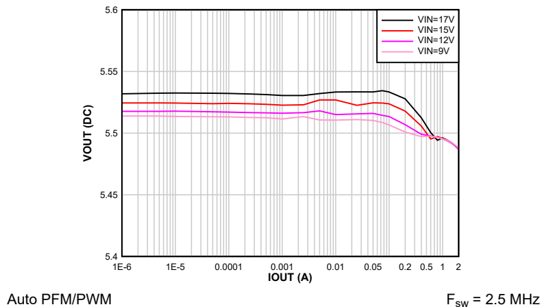
Figure 8-60. Output Voltage vs Output Current V OUT = 5.5 V
