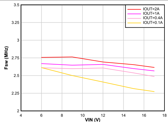
Figure 8-20. Switching Frequency vs Input Voltage V_{OUT} = 1.2 \text{ V}
