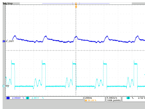
Vout = 0.9 V IOUT = 1 A Figure 9-28. PWM-DCM Operation TPSM8287A12BBS
