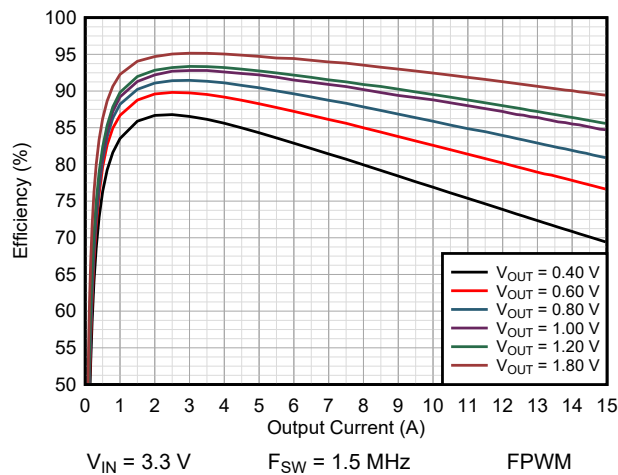
Figure 9-16. Efficiency TPSM8287A15BAH
