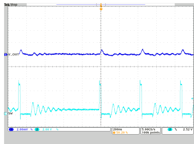
Vout = 0.9 V IOUT = 100 mA Figure 9-29. PFM-DCM Operation TPSM8287A12BBS
