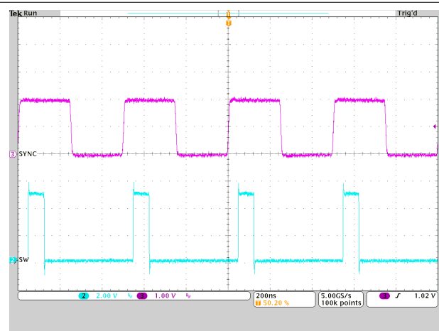
IOUT = 1 A f (SYNC) = 2 MHz Figure 9-31. Synchronization to an External Clock
