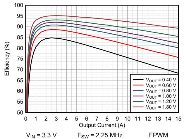
Figure 9-17. Efficiency TPSM8287A15BBH
