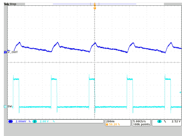
Vout = 0.9 V IOUT = 2 A Figure 9-27. PWM-CCM Operation TPSM8287A12BBS
