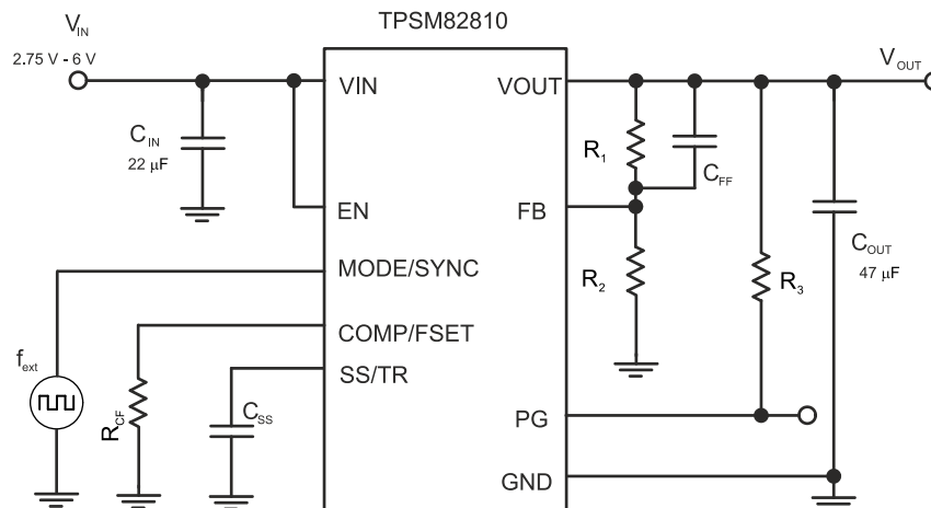
Figure 9-35. Frequency Synchronization
