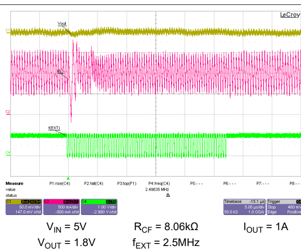
Figure 9-37. Applying and Removing the Synchronization Signal (FPWM)
