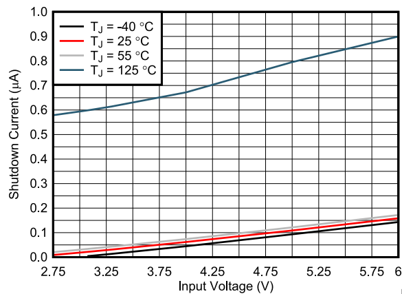
Figure 6-2. Shutdown Current
