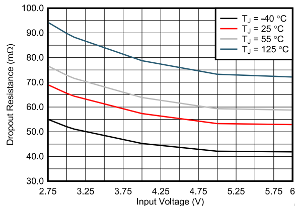
Figure 6-4. Dropout Resistance
