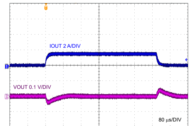
Figure 9-14. Load Transient, 0 A to 1.5 A
