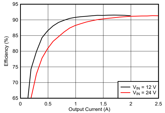
Figure 9-12. Efficiency
