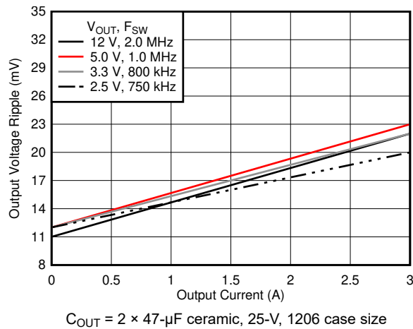
Figure 7-15. Output Voltage Ripple
