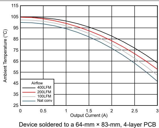
Figure 7-24. Safe Operating Area V_{OUT} = 12\text{ V} , f_{SW} = 2\text{ MHz}
