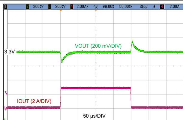
Figure 9-4. Load Transient, 0 A to 3 A, 1 A/μs
