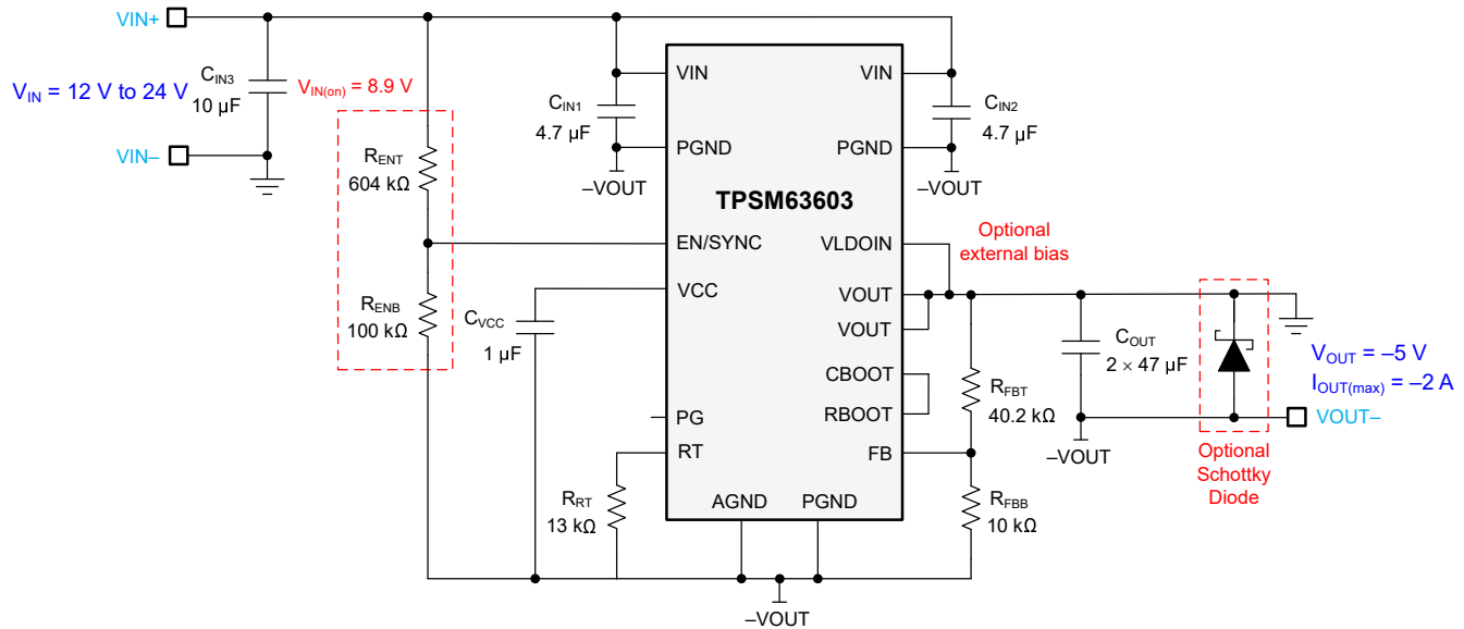
Figure 8-12. Circuit Schematic
