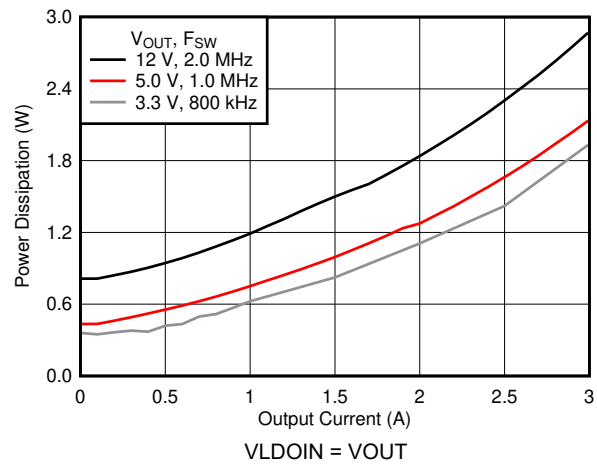
Figure 6-20. Power Dissipation
