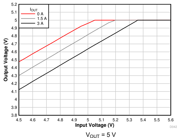
Figure 7-9. Voltage Dropout
