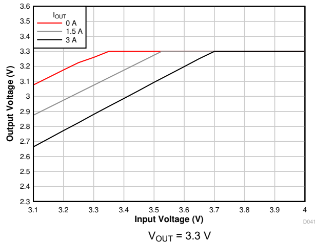
Figure 7-7. Voltage Dropout
