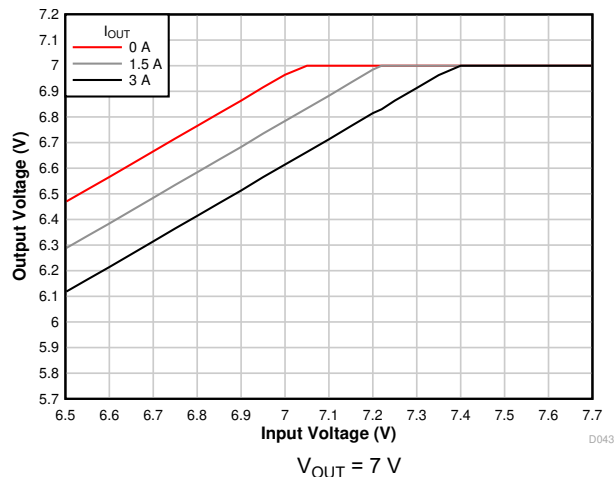
Figure 7-11. Voltage Dropout
