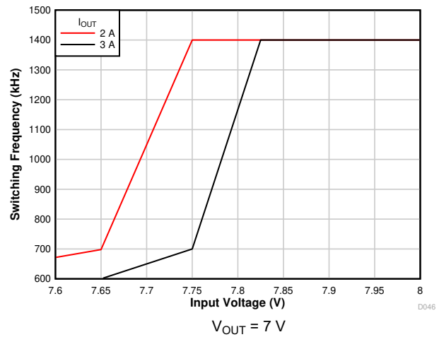
Figure 7-12. Frequency Foldback
