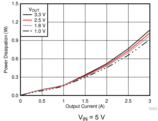
Figure 6-3. Power Dissipation versus Output Current
