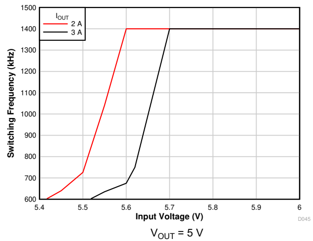
Figure 7-10. Frequency Foldback
