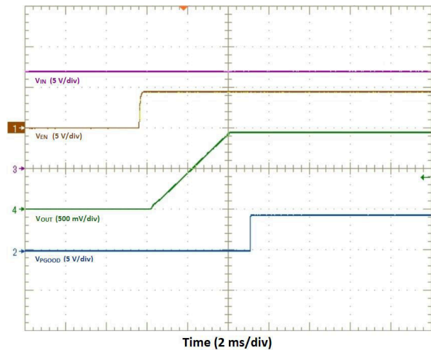
Figure 8-3. Start-Up Waveforms
