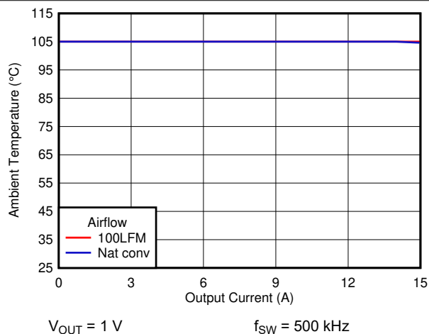
Figure 6-10. Safe Operating Area
