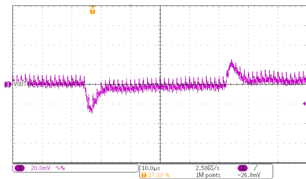
Figure 8-5. 10-A Transient Load Step
