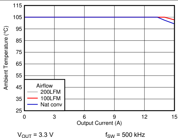
Figure 6-12. Safe Operating Area
