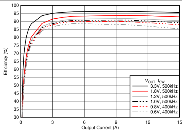
Figure 6-7. Efficiency vs Output Current
