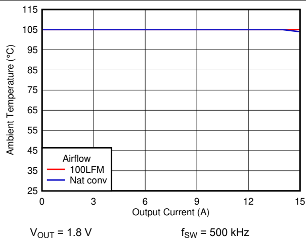
Figure 6-11. Safe Operating Area
