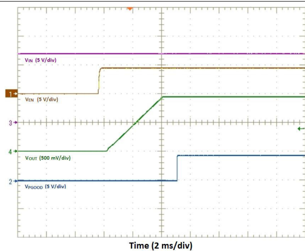
Figure 8-3. Start-Up Waveforms
