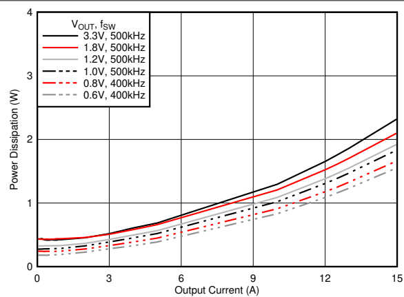
Figure 6-8. Power Dissipation vs Output Current
