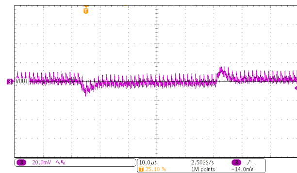
Figure 8-4. 5-A Transient Load Step
