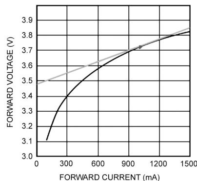
Figure 18. Dynamic Resistance
