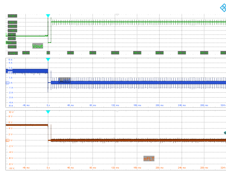
Ch2: Output voltage (4 V/div); Ch3: LED current (1 A/div); Ch4: FLT voltage (2 V/div); Time: 40 ms/div
