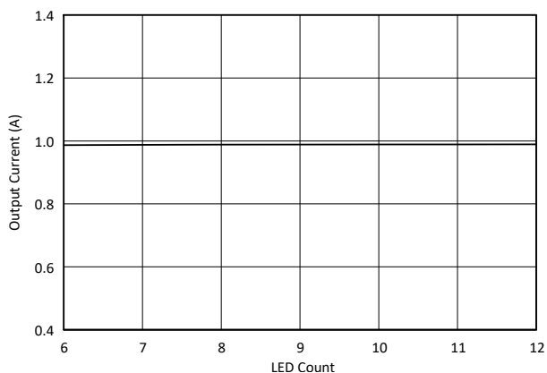
Figure 6-2. Output Current vs. LED Count
