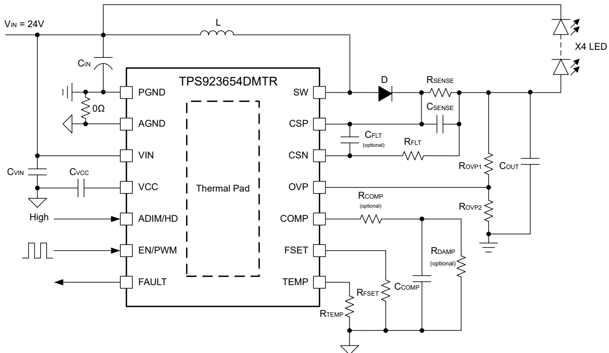
Figure 8-12. Buck-Boost, 24V Input, 2A Output, 4-piece WLED, PWM Dimming Reference Design
