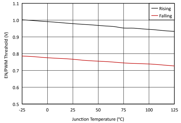
Figure 6-10. EN/PWM Threshold vs. Junction Temperature
