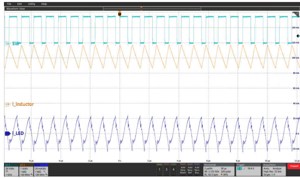
Figure 8-13. LED Current Ripple at PWM_{ADIM} = 100\% , 1kHz and F_{SW} = 1.2MHz
