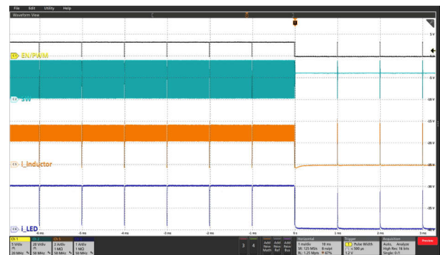
Figure 8-16. LED PWM Dimming at PWM_{PWM} = 1\% , 1kHz
