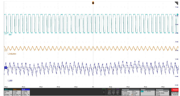
Figure 8-3. LED Current Ripple at DIM_{Analog} = 0.2V and F_{SW} = 400kHz
