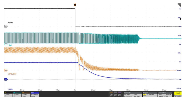
Figure 8-5. LED Current Transient for a DIM_{Analog} Transition from 2V to 0.2V
