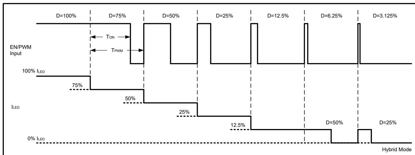
Figure 7-3. Hybrid Dimming
