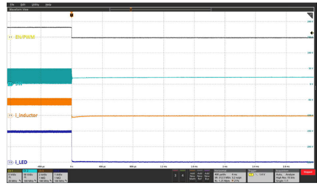
Figure 8-22. Shutdown at PWM PWM = 100%, 20kHz
