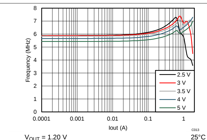
Figure 12. Switching Frequency vs Output Current
