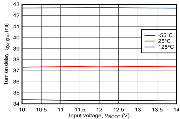
Figure 6-15. High-Side Turn On Delay vs Input Voltage V_{IN} (IIM)
