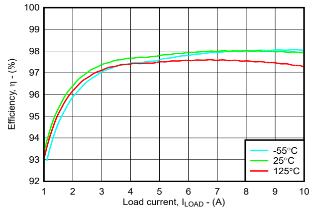
Figure 6-44. 100V to 28V Efficiency
