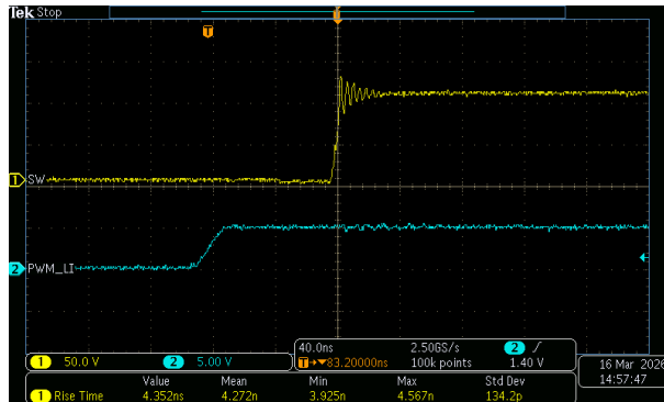
Figure 9-2. 100V Switch Node Rising
