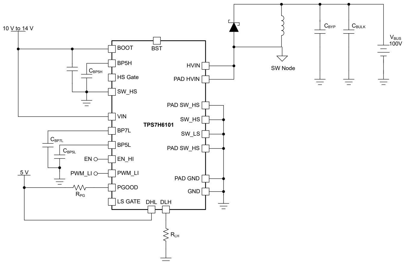
Figure 9-5. High Side Double Pulse Test Configuration
