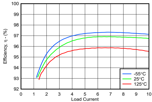
Figure 6-44. 100V to 28V Efficiency
