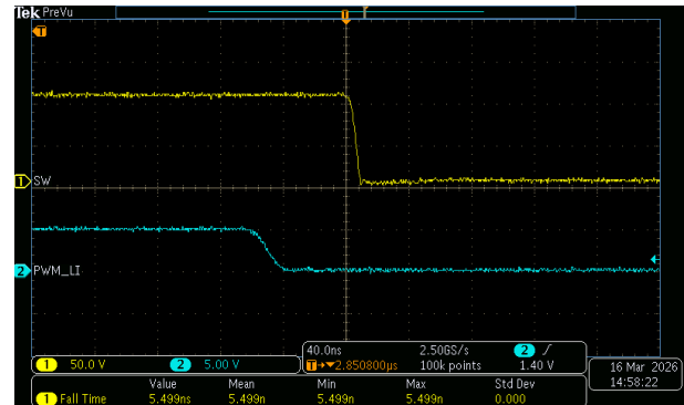
Figure 9-3. 100V Switch Node Falling
