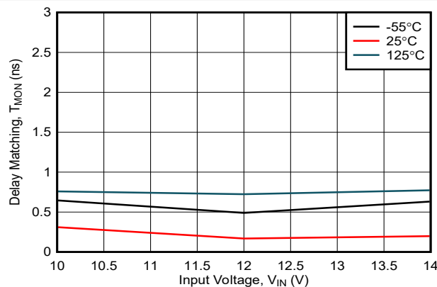
Figure 6-23. Delay Matching Low-Side On and High-Side Off vs Input Voltage
