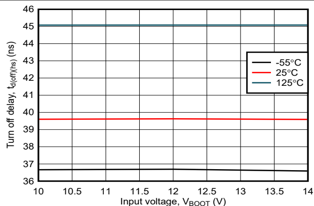
Figure 6-17. High-Side Turn Off Delay vs Input Voltage V_{IN} (IIM)
