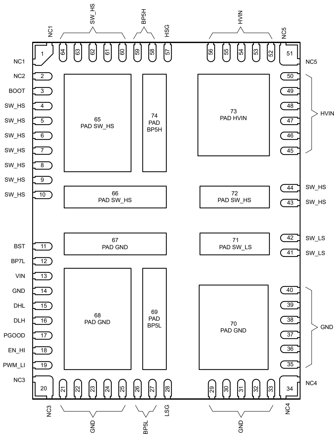
Figure 5-1. NPR Package 64-Pin LGA (Top View)
