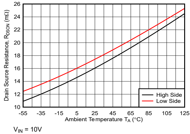
Figure 6-1. On-Resistance vs Junction Temperature (High-Side and Low-Side)
