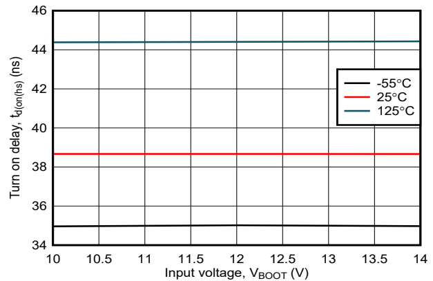
Figure 6-16. High-Side Turn On Delay vs Input Voltage V_{IN} (PWM)
