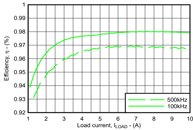
Figure 6-43. 100V to 28V Efficiency
