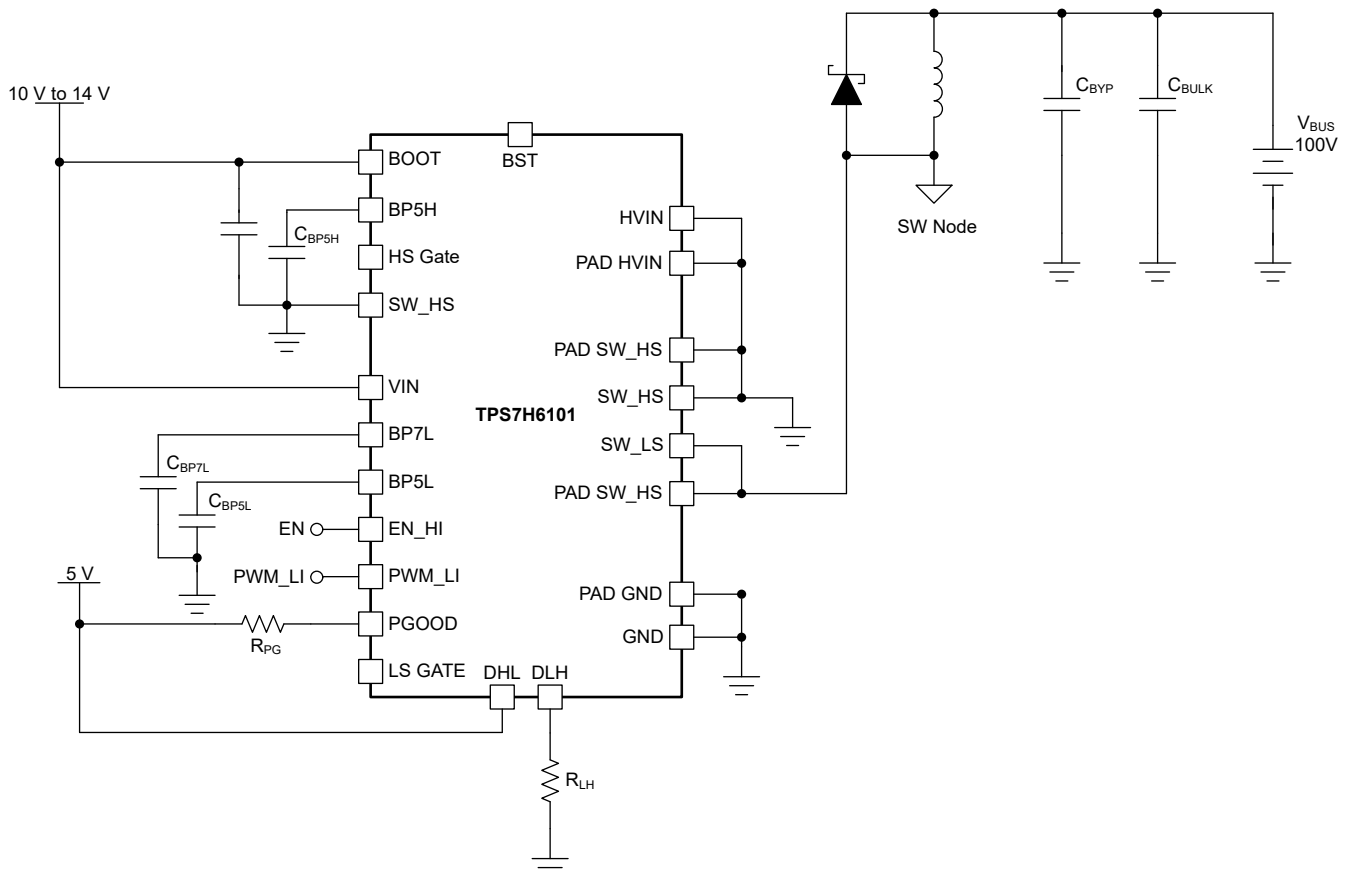
Figure 9-4. Low Side Double Pulse Test Configuration
