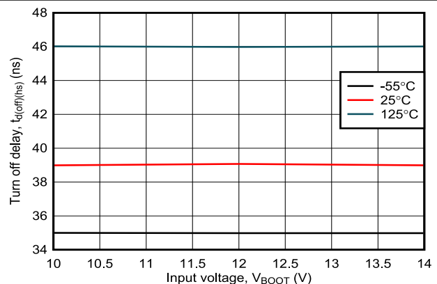
Figure 6-18. High-Side Turn Off Delay Voltage vs Input Voltage V_{IN} (PWM)
