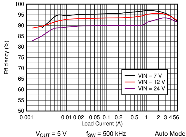
Figure 8-3. TPS7H4010-SEP Efficiency
