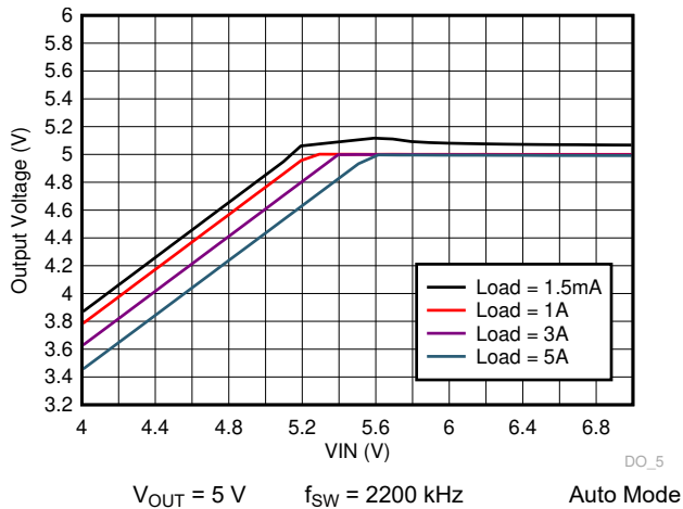
Figure 8-11. TPS7H4010-SEP Dropout Curve
