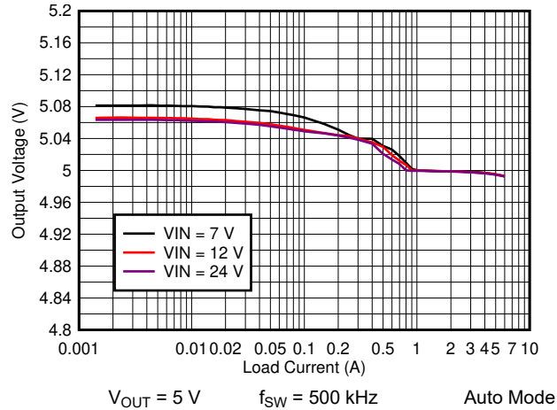
Figure 8-9. TPS7H4010-SEP Load and Line Regulation
