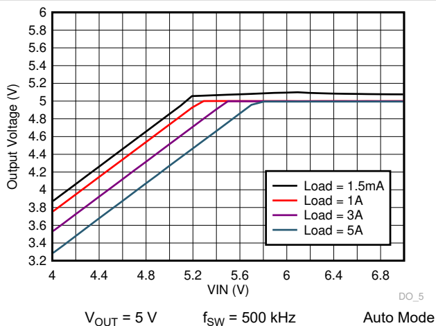
Figure 8-13. TPS7H4010-SEP Dropout Curve
