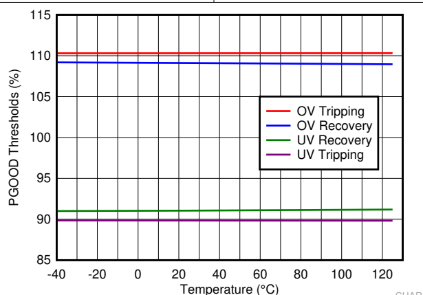
Figure 6-9. PGOOD Thresholds
