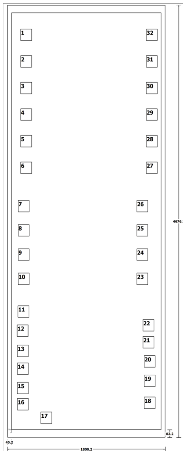
Figure 5-2. TPS7H4010-SEP Bare Die Diagram
