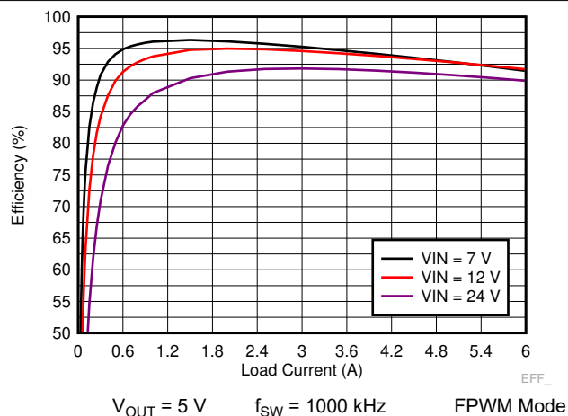
Figure 8-6. TPS7H4010-SEP Efficiency
