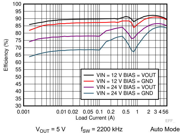
Figure 7-6. TPS7H4010 Efficiency Comparison With Bias = V_{OUT} to Bias = GND in Auto Mode
