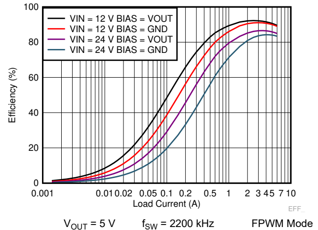
Figure 7-7. TPS7H4010 Efficiency Comparison With Bias = V_{OUT} to Bias = GND in FPWM Mode
