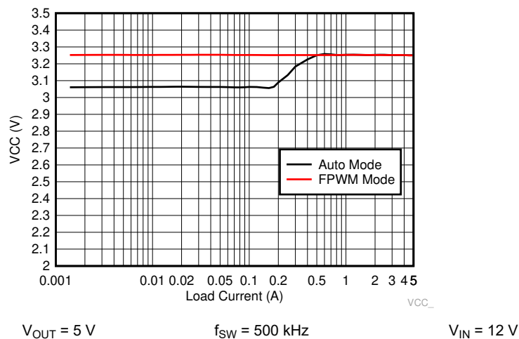
Figure 7-8. VCC Voltage vs Load Current
