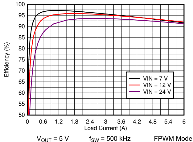
Figure 8-4. TPS7H4010-SEP Efficiency
