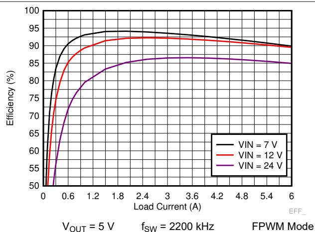
Figure 8-8. TPS7H4010-SEP Efficiency
