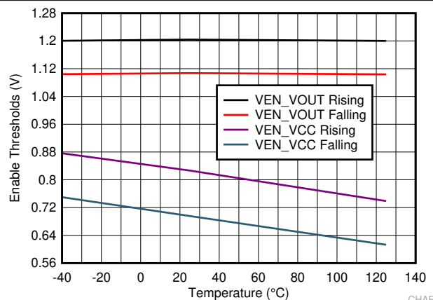
Figure 6-8. Enable Thresholds
