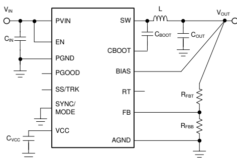
Simplified Schematic
