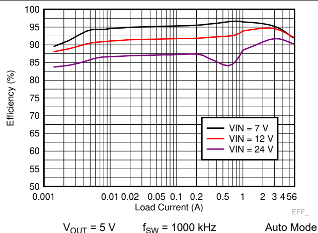
Figure 8-5. TPS7H4010-SEP Efficiency
