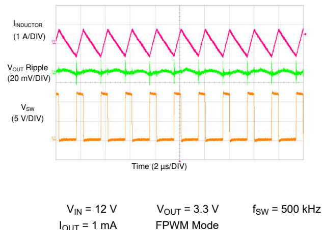
Figure 8-18. TPS7H4010-SEP Switching Waveform and V_{OUT} Ripple
