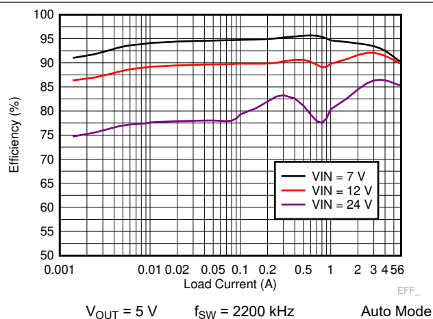
Figure 8-7. TPS7H4010-SEP Efficiency
