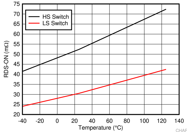
Figure 6-1. High-Side and Low-Side Switches R_{DS-ON}
