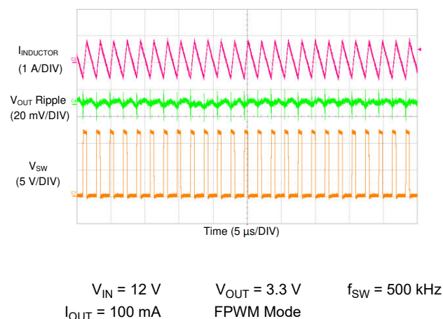
Figure 8-20. TPS7H4010-SEP Switching Waveform and V_{OUT} Ripple
