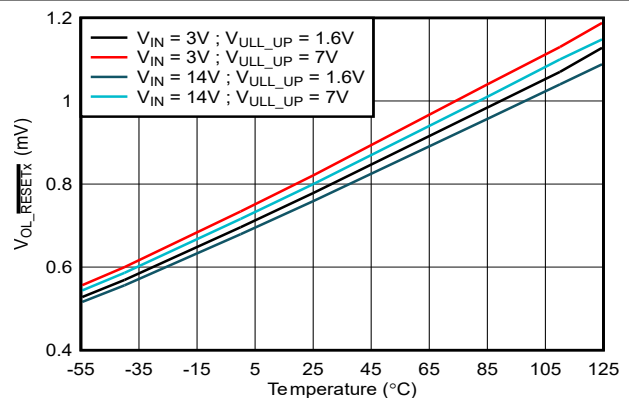
Figure 6-36. RESET1 VOL Voltage vs Temperature Across V_{PULL\_UP} and V_{IN} at I_{LOAD} = 10mA for the TPS7H3124
