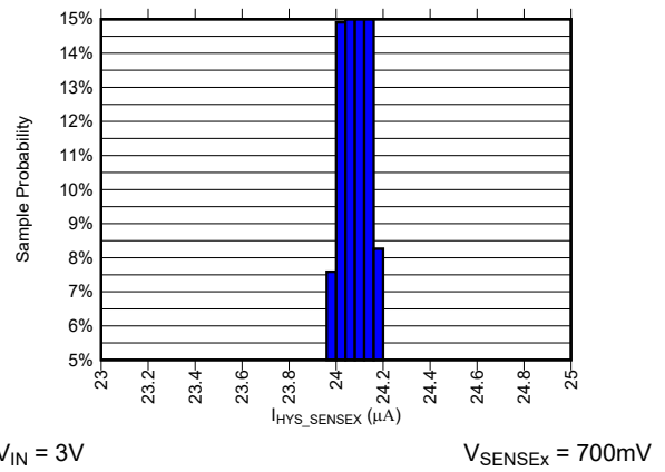
Figure 6-10. I_{HYS\_SENSEx} Current Distribution at Temperature of -55^{\circ}C
