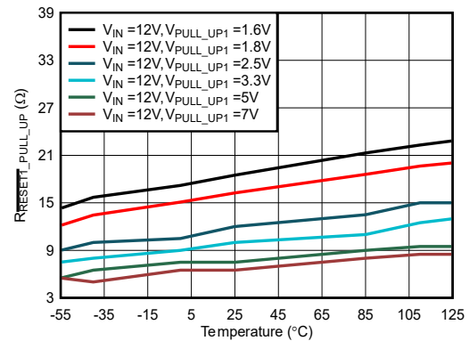
Figure 6-28. RESET1 Pull-Up Resistance vs Temperature Across V_{PULL\_UP1} at I_{LOAD} = 2mA
