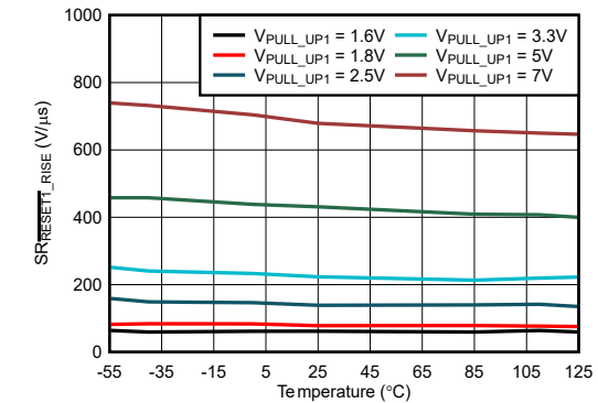
Figure 6-18. SR_{RESET1\_RISE} vs Temperature Across V_{PULL\_UP1}
