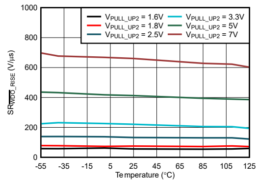
Figure 6-22. SR_{WDO\_RISE} vs Temperature Across V_{PULL\_UP2}
