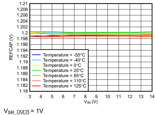
Figure 6-14. REFCAP vs V_{IN} Across Temperature
