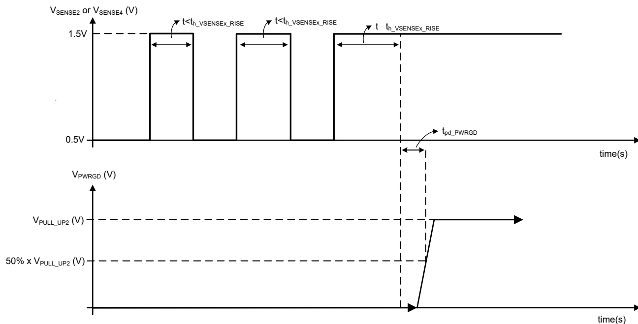
Figure 7-16. VSENSE2 and VSENSE4 Rising Threshold Hold Time ( t_{th\_VSENSEx\_RISE} )
