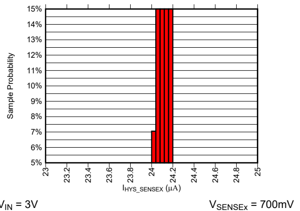
Figure 6-12. I_{HYS\_SENSEx} Current Distribution at Temperature of 125^{\circ}C
