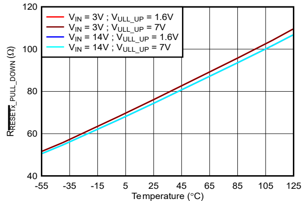
Figure 6-34. RESET1 Pull-Down Resistance vs Temperature Across V_{PULL\_UP} and V_{IN} at I_{LOAD} = 2mA for the TPS7H3124
