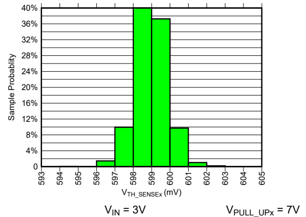
Figure 6-8. V_{TH\_SENSEx} Voltage Distribution at Temperature of +25^{\circ}C
