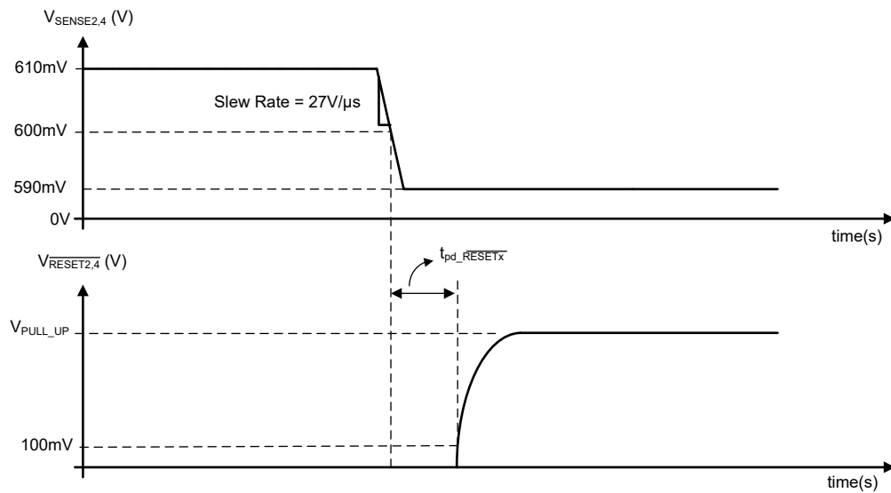
Figure 7-6. \overline{\text{RESET2}} and \overline{\text{RESET4}} Propagation Delay ( t_{\text{pd\_RESETx}} ) Time Measurement for TPS7H31x4 (Open-Drain)
