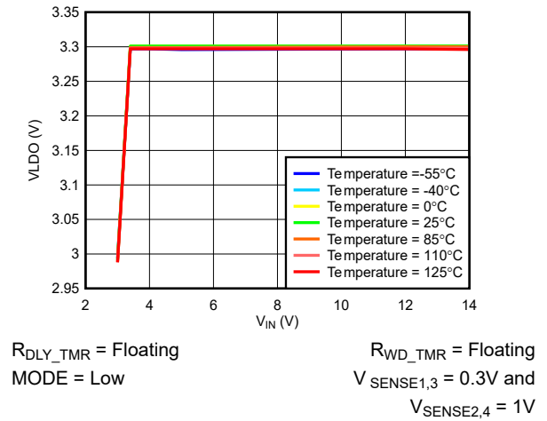
Figure 6-16. VLDO vs V_{IN} Across Temperature
