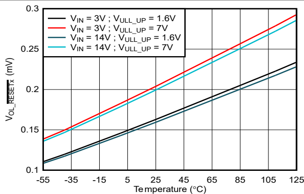
Figure 6-35. RESET1 VOL Voltage vs Temperature Across V_{PULL\_UP} and V_{IN} at I_{LOAD} = 2mA for the TPS7H3124
