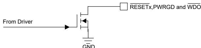
Figure 8-17. \overline{\text{RESETx}} , PWRGD and \overline{\text{WDO}} Outputs in Open-Drain
