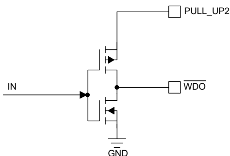
Figure 8-15. \overline{\text{WDO}} Push-Pull Output Stage for UV Channel Type
