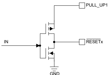
Figure 8-13. \overline{\text{RESETx}} Push-Pull Output Stages for UV Channel Type
