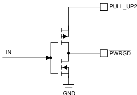
Figure 8-14. PWRGD Push-Pull Output Stage for UV Channel Type
