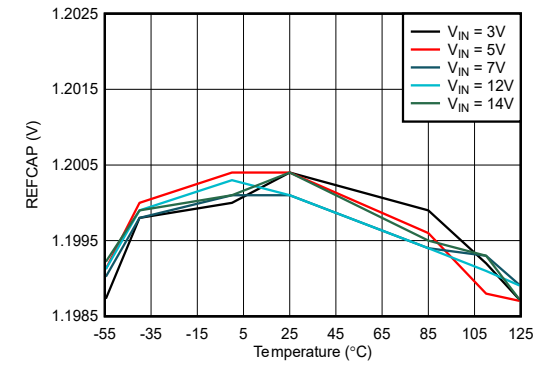
Figure 6-15. REFCAP vs Temperature Across V_{IN}
