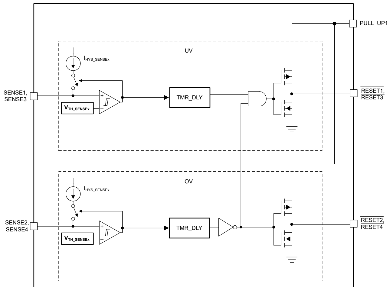
Figure 8-11. Window Comparator for TPS7H3024 when \text{MODE}=1
