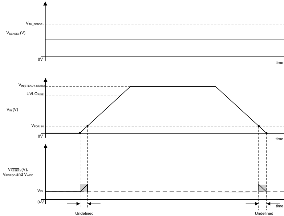
Figure 8-3. Outputs in a Valid Low State After V_{IN} > V_{POR\_IN}
