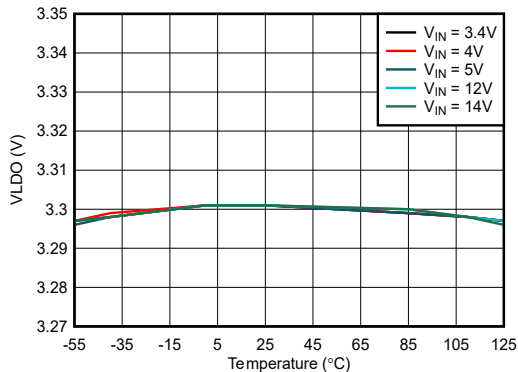
Figure 6-17. VLDO vs Temperature Across V_{IN}
