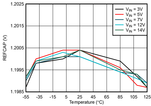
Figure 6-15. REFCAP vs Temperature Across V_{IN}
