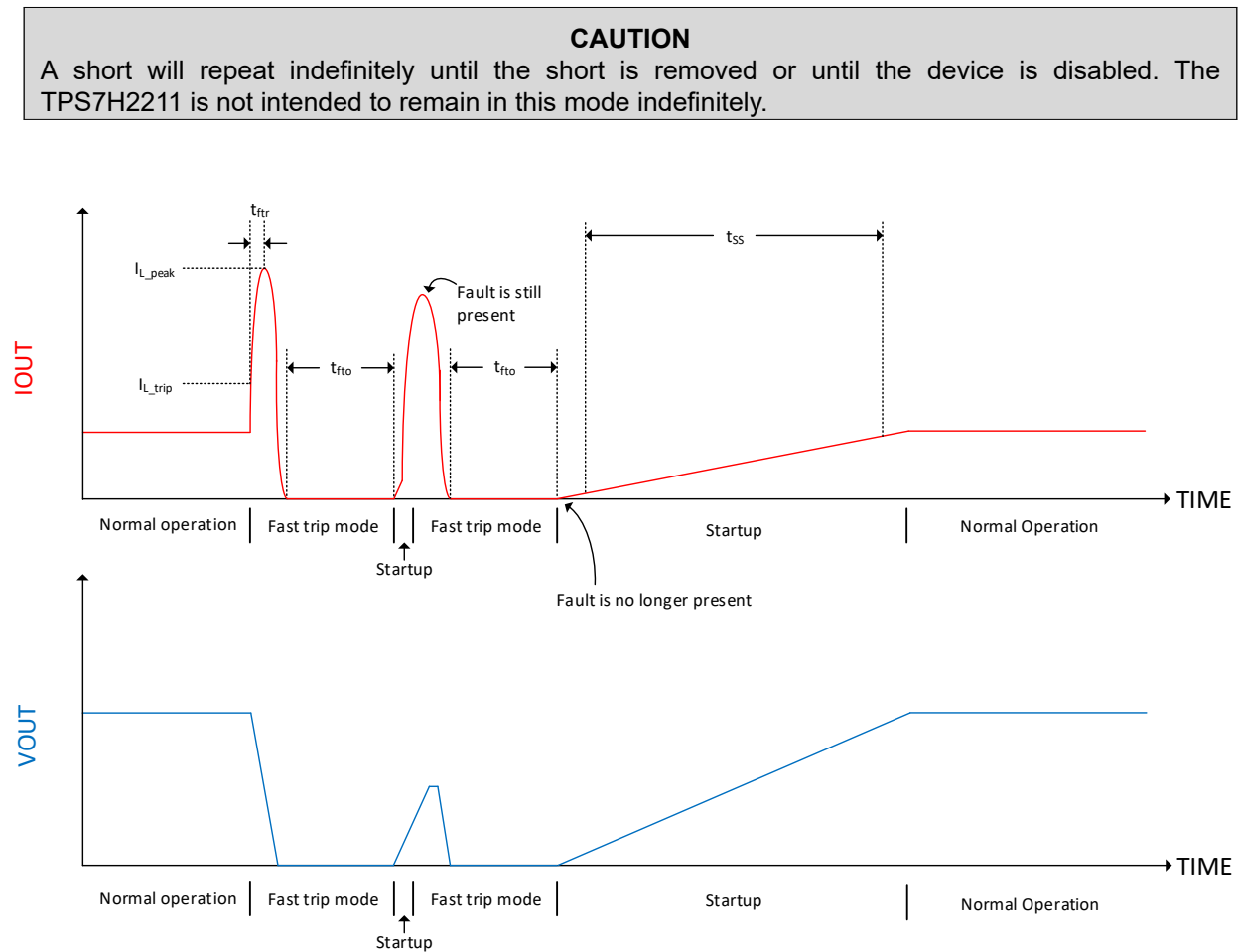
Figure 9-5. Two Hard Shorts and Recovery
