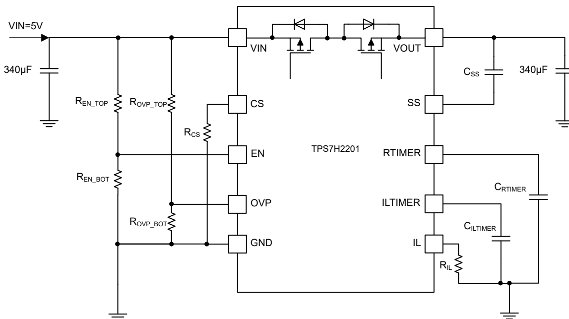
Figure 9-3. Typical Application Schematic
