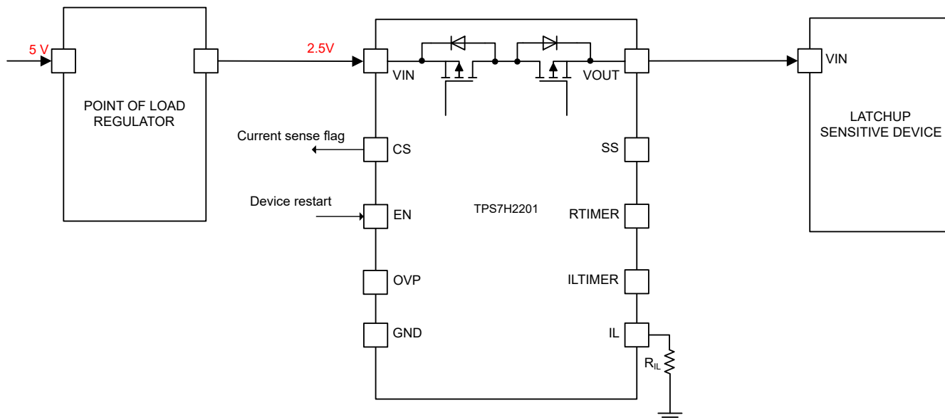
Figure 9-2. Protection Example Using the TPS7H2201
