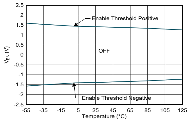
Figure 6-12. Enable Threshold Voltage vs Temperature
