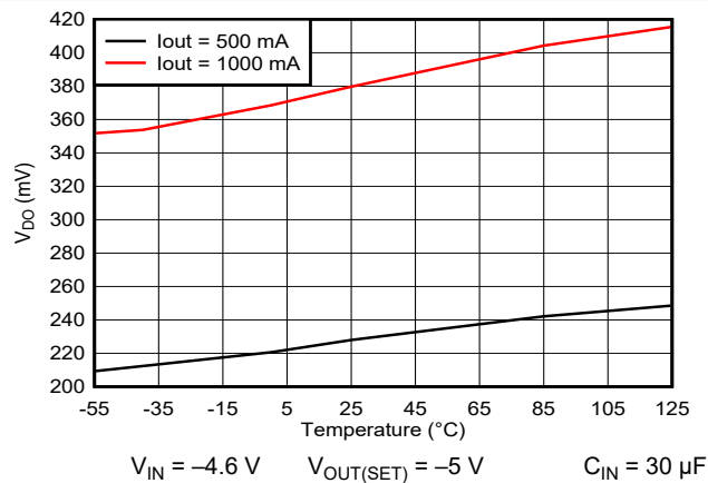
Figure 6-11. Dropout Voltage vs Temperature Across Output Current
