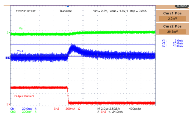
Figure 21. Expanded View Overshoot
