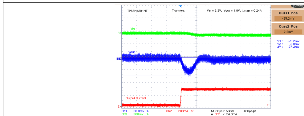
Figure 22. Expanded View Undershoot
