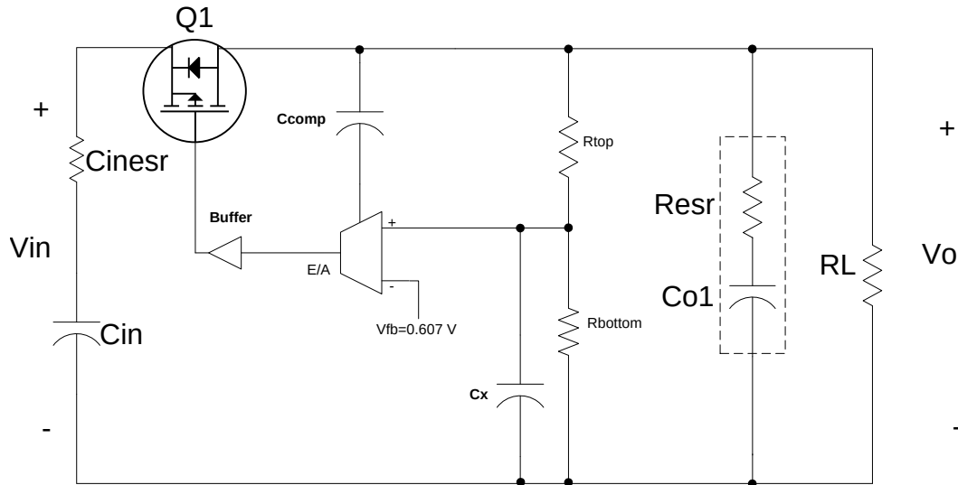
Figure 25. TPS7H1201-HT Compensation
