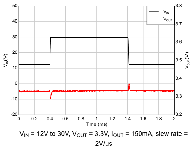
Figure 7-6. Line Transient
