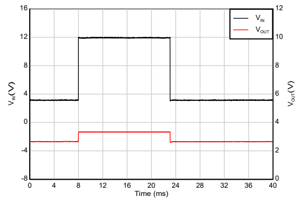
Figure 5-32. Line Transient
