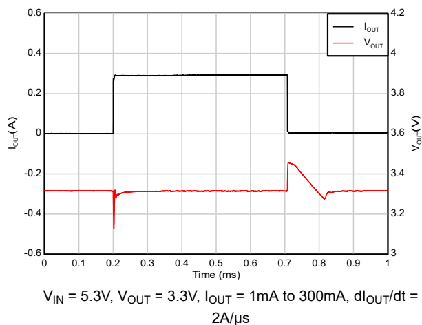
Figure 7-11. Load Transient (1mA to 300mA)
