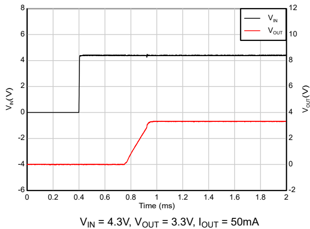
Figure 7-7. Start-up with EN & V_{IN} tied together
