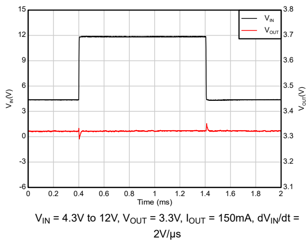
Figure 7-9. Line Transient (4.3V to 12V)
