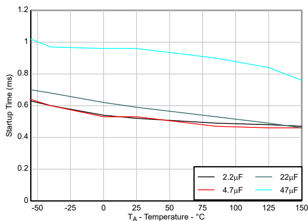
Figure 5-21. Start-up Time vs C_{OUT}
