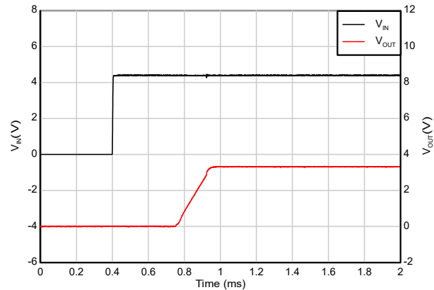
Figure 7-6. Start-up with EN & V_{IN} tied together
