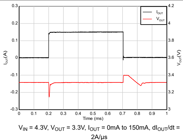
Figure 5-47. Load Transient (0mA to 150mA)
