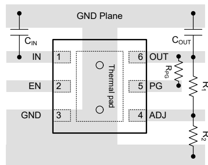
Figure 7-17. Example Layout for TPS7E66-Q1 DRV Package
