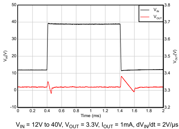
Figure 5-45. Line Transient (12V to 40V)
