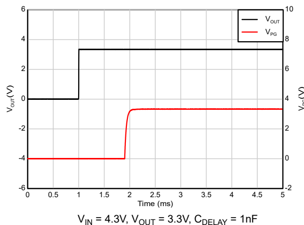
Figure 5-41. PG Delay with C_{DELAY} = 1\text{nF}
