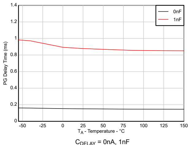
Figure 5-19. PG Delay time vs Temperature
