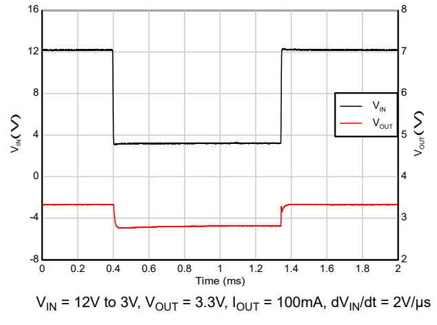
Figure 7-12. Dropout Recovery (12V to 3V)
