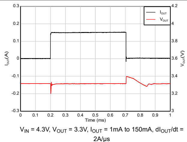
Figure 5-48. Load Transient (1mA to 150mA)
