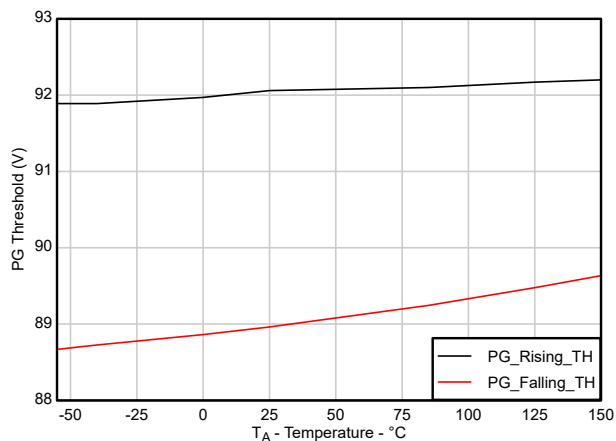
Figure 5-18. PG Threshold ( V_{IT+(PG)}/V_{IT-(PG)} ) vs Temperature
