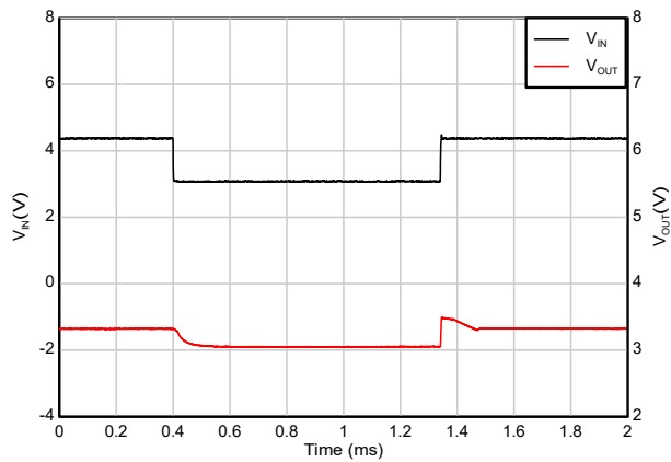
Figure 5-49. Dropout Recovery (4.3V to 3V)
