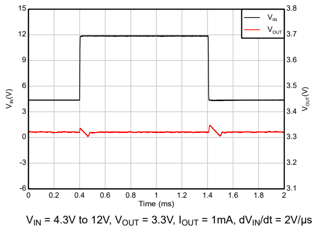
Figure 5-43. Line Transient (4.3V to 12V)
