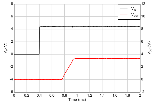
Figure 5-32. Start-up with EN & V_{IN} tied together
