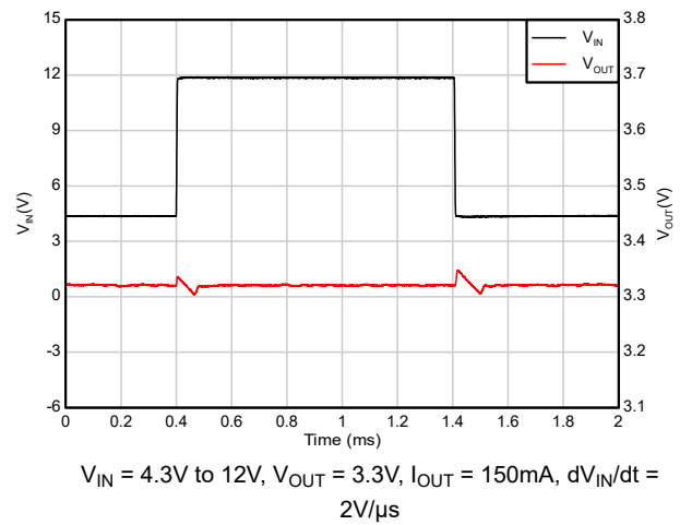
Figure 5-44. Line Transient (4.3V to 12V)
