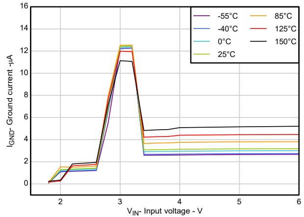
Figure 5-8. I_{GD} vs V_{IN}
