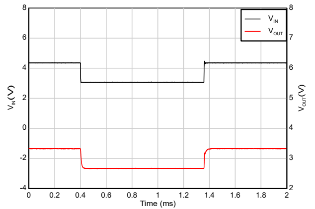
Figure 5-50. Dropout Recovery (4.3V to 3V)
