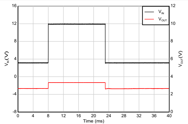
Figure 5-52. Dropout Recovery (12V to 3V)
