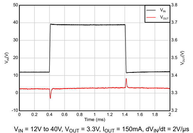
Figure 5-46. Line Transient (12V to 40V)
