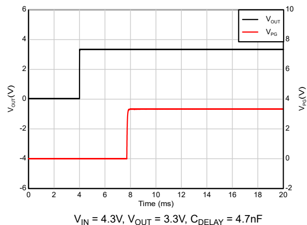
Figure 5-42. PG Delay with C_{DELAY} = 4.7\text{nF}
