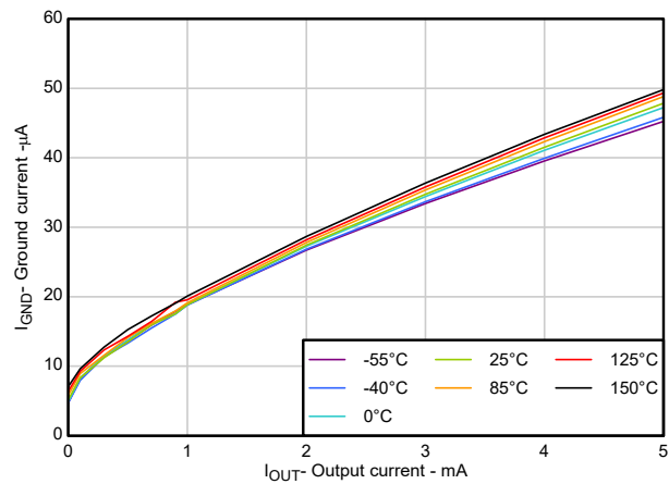
Figure 5-9. I_{GD} vs I_{OUT}
