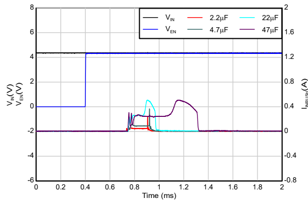
Figure 5-31. Inrush Current vs C_{OUT}
