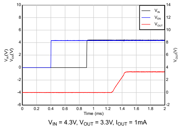
Figure 5-38. Start-up with sequencing ( V_{IN} after EN)
