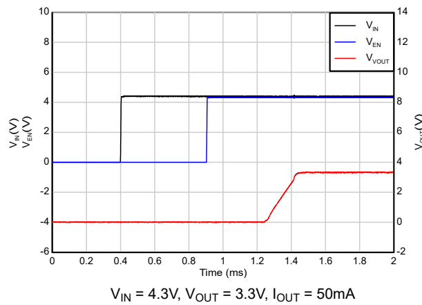
Figure 5-37. Start-up with sequencing (EN after V_{IN} )
