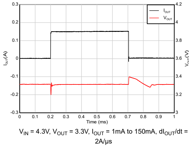
Figure 7-11. Load Transient (1mA to 150mA)
