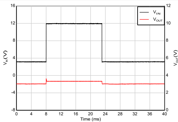
Figure 5-51. Dropout Recovery (12V to 3V)
