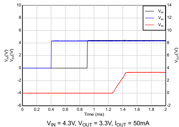
Figure 5-40. Start-up with sequencing ( V_{IN} after EN)
