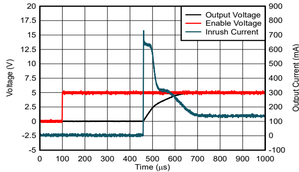
Figure 7-8. Power-Up Waveform With EN
