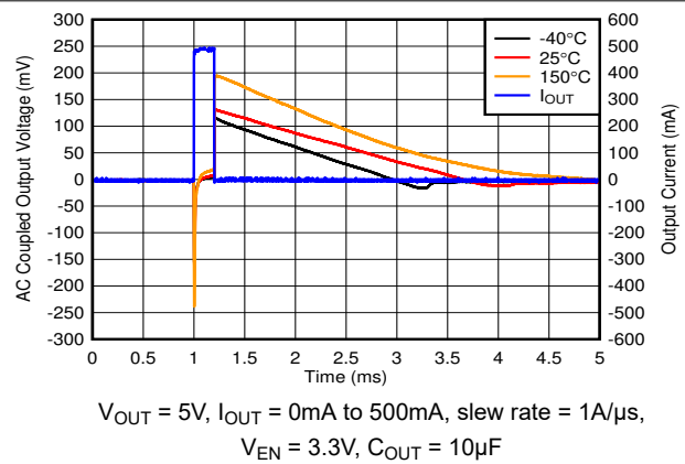
Figure 5-24. Load Transient, No Load to 500mA
