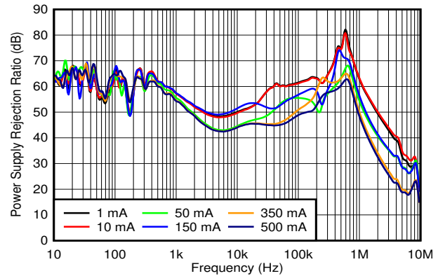
Figure 7-9. PSRR
