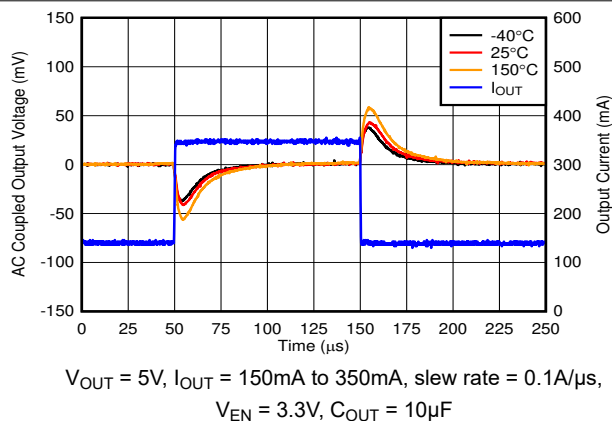
Figure 5-23. Load Transient, 150mA to 350mA
