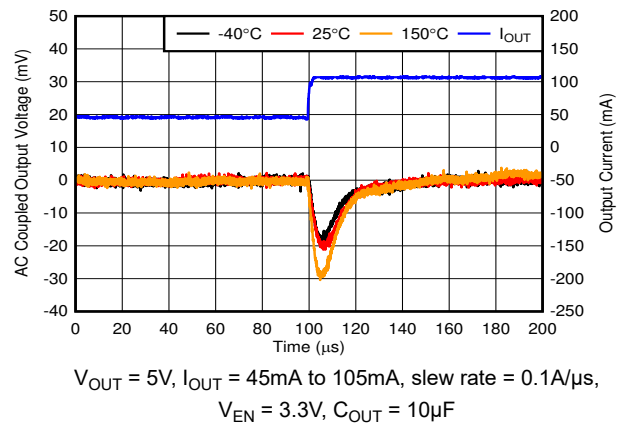
Figure 5-20. Load Transient, 45mA to 105mA Rising Edge
