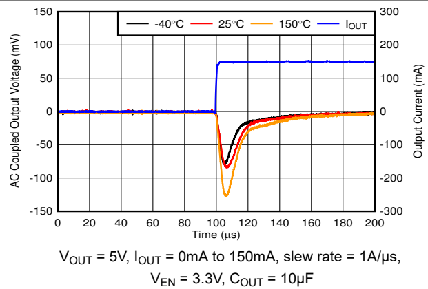
Figure 5-22. Load Transient, No Load to 150mA Rising Edge
