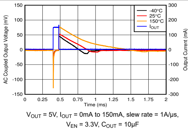
Figure 5-21. Load Transient, No Load to 150mA
