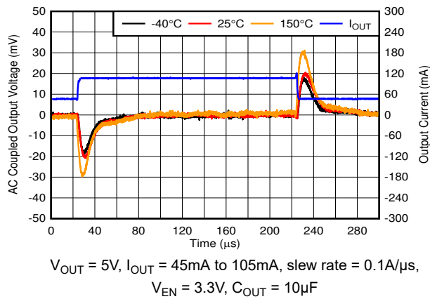
Figure 5-19. Load Transient, 45mA to 105mA
