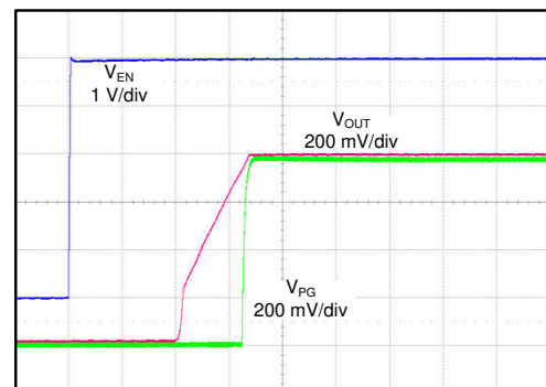
Figure 5-32. Start-Up ( SS\_CTRL = \text{GND} , C_{NR/SS} = 0\text{nF} )
