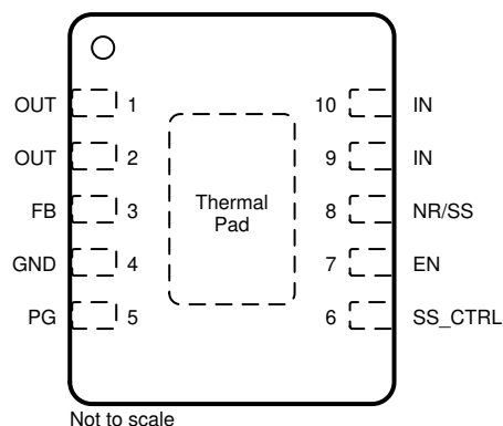
Figure 4-1. DSK Package, 2.5mm × 2.5mm, 10-Pin WSON (Top View)
