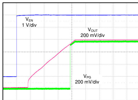
Figure 5-33. Start-Up ( SS\_CTRL = \text{GND} , C_{NR/SS} = 10\text{nF} )
