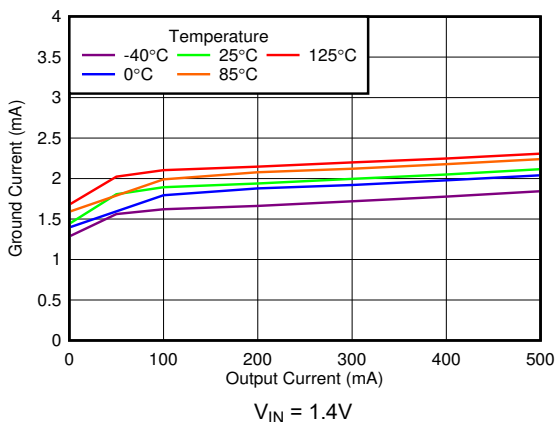
Figure 5-19. Ground Current vs Output Current
