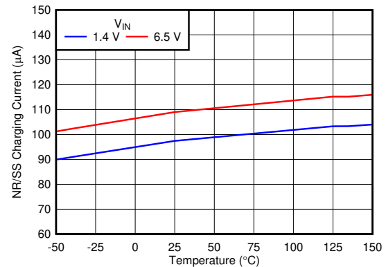
Figure 5-26. Soft-Start Current vs Temperature ( SS\_CTRL = V_{IN} )
