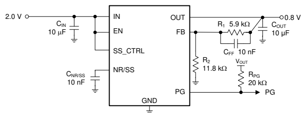
Typical Application Circuit
