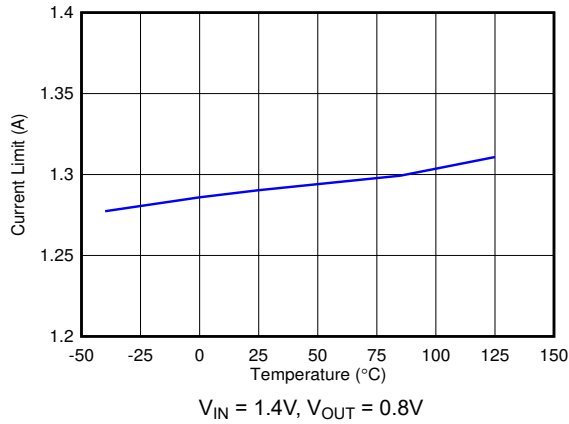
Figure 5-13. Current Limit vs Temperature
