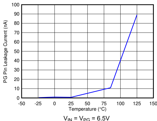
Figure 5-24. PG Leakage Current vs Temperature
