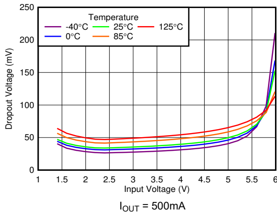
Figure 5-15. Dropout Voltage vs Input Voltage
