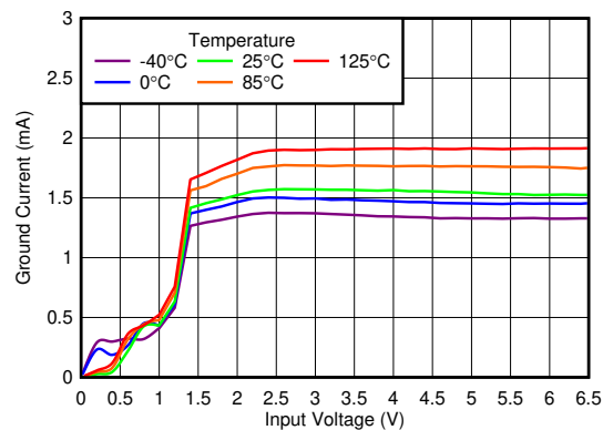
Figure 5-20. Ground Current vs Input Voltage
