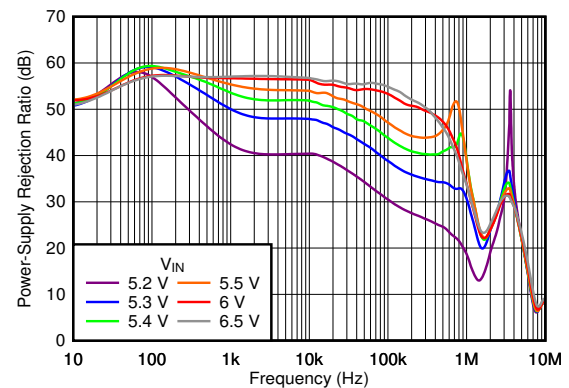
Figure 5-2. PSRR vs Frequency and Input Voltage
