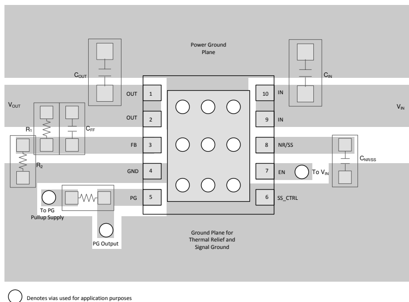
Figure 7-5. TPS7A90 Example Layout
