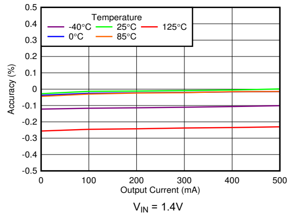
Figure 5-16. Load Regulation
