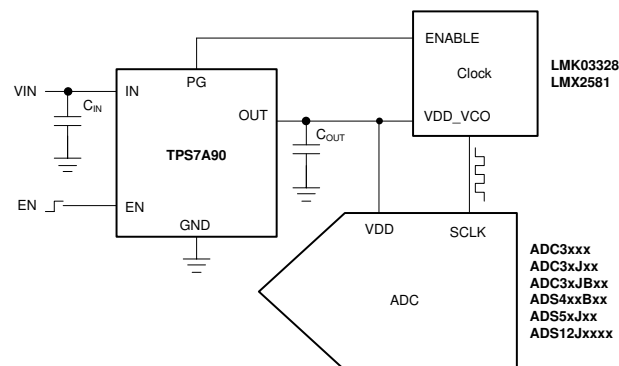
Typical Application Diagram
