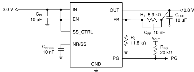
Figure 7-2. Application Example
