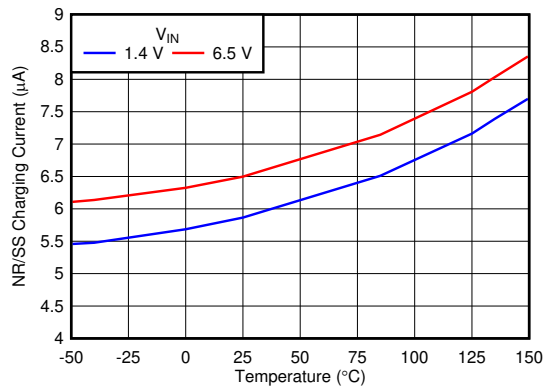
Figure 5-25. Soft-Start Current vs Temperature ( SS\_CTRL = \text{GND} )
