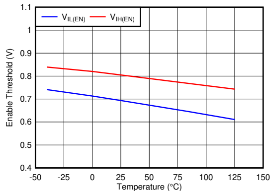
Figure 5-27. Enable Threshold vs Temperature
