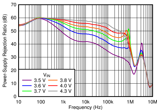
Figure 5-1. PSRR vs Frequency and Input Voltage
