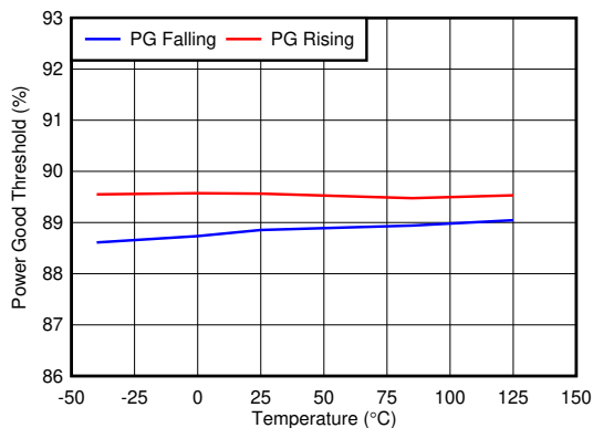
Figure 5-23. PG Threshold vs Temperature
