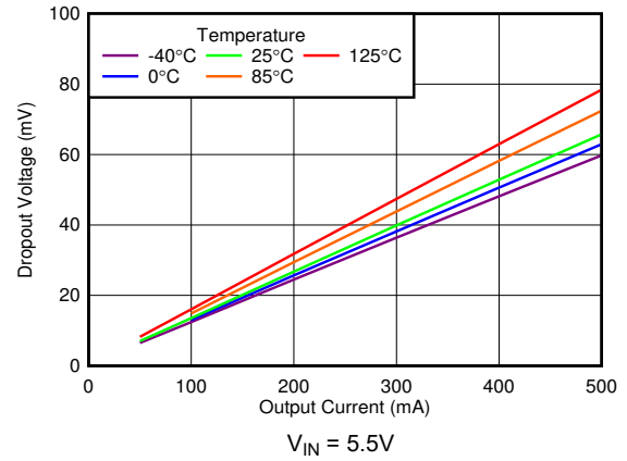
Figure 5-14. Dropout Voltage vs Output Current
