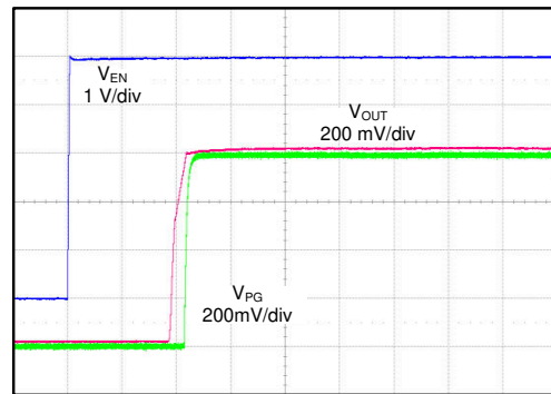
Figure 5-32. Start-Up ( SS\_CTRL = \text{GND} , C_{NR/SS} = 0\text{nF} )
