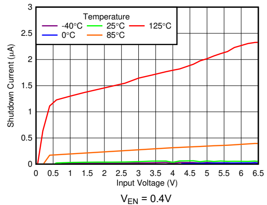
Figure 5-18. Shutdown Current vs Input Voltage
