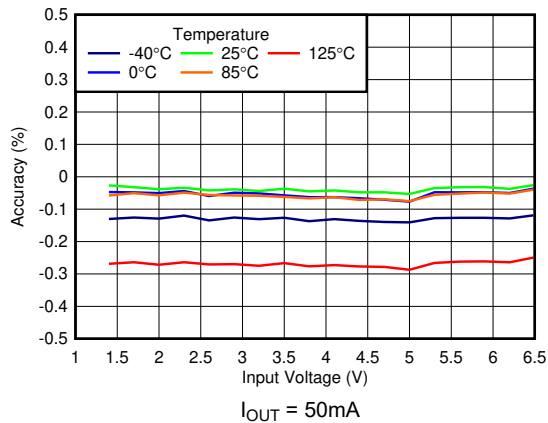
Figure 5-17. Line Regulation
