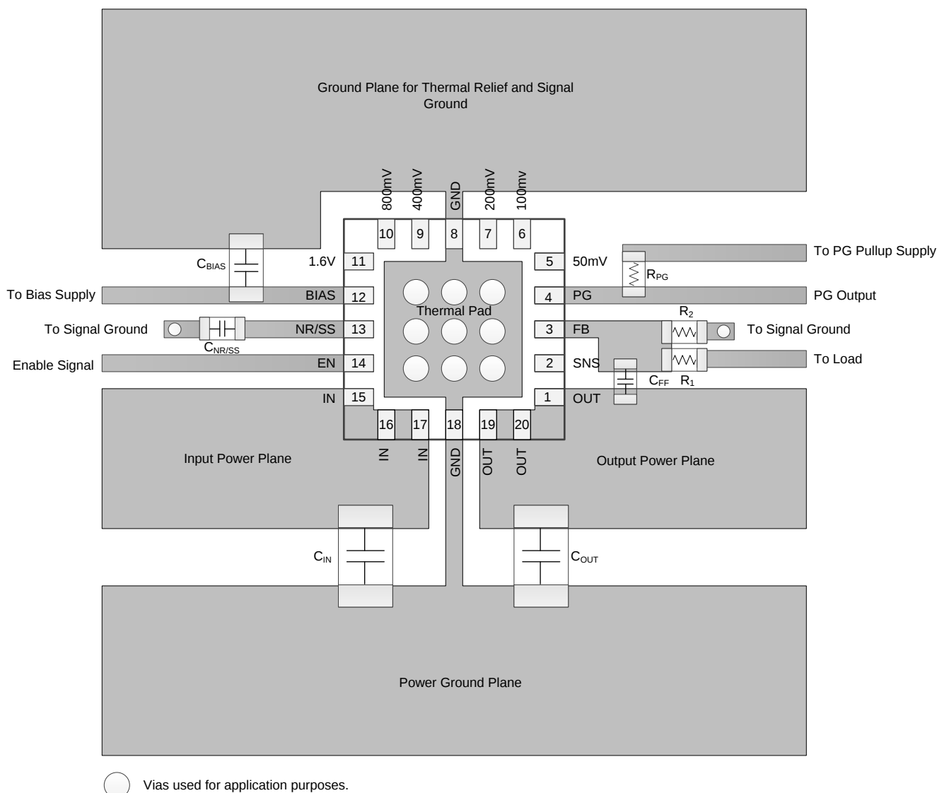
Figure 71. Example Layout
