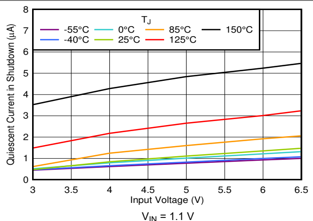
Figure 7-60. Shutdown Current vs Bias Voltage
