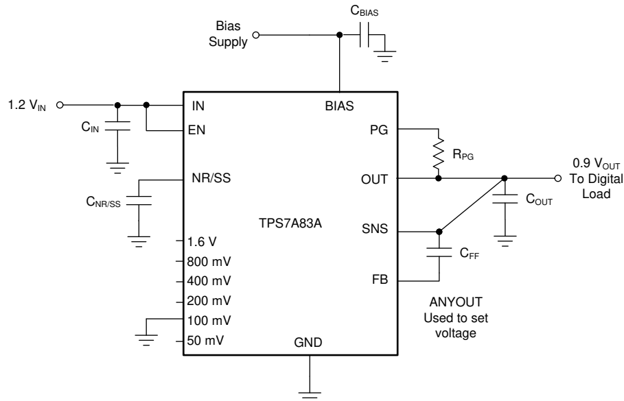
Figure 9-21. TPS7A83A Typical Application: Low-Input, Low-Output (LILLO) Voltage Conditions
