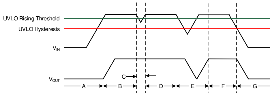
Figure 9-4. Typical UVLO Operation
