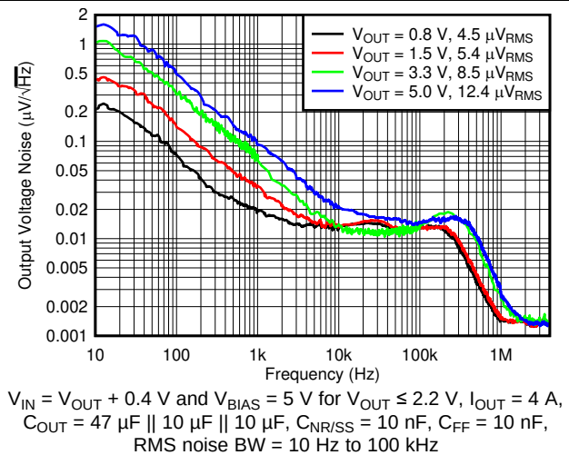
Figure 10. Output Voltage Noise vs Frequency and V_{OUT}
