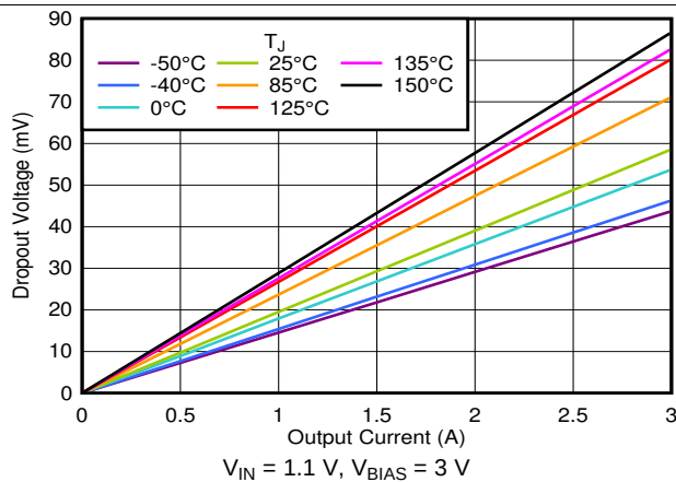
Figure 23. Dropout Voltage vs Output Current With Bias
