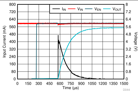
Figure 5-85. Inrush Current
