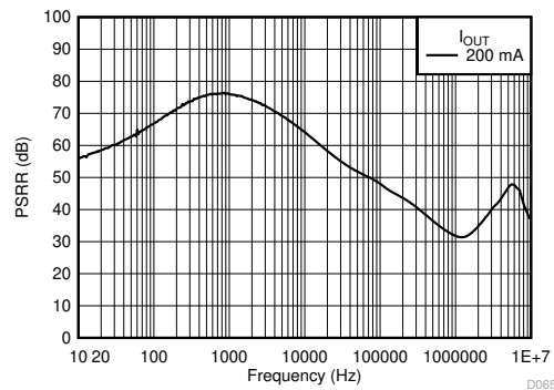
Figure 7-6. PSRR
