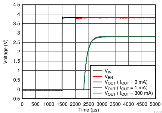
Figure 5-75. Start-Up
