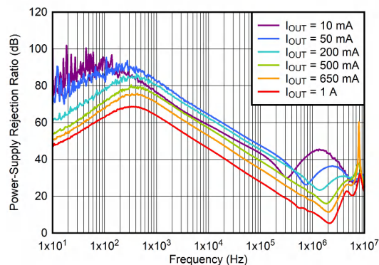
Figure 5-26. PSRR vs Frequency and I_{\text{OUT}}
