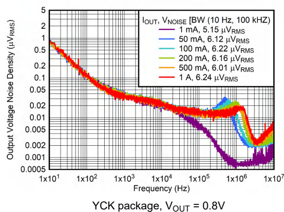
Figure 5-28. Output Noise vs Frequency and I_{\text{OUT}}
