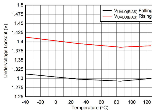
Figure 5-14. V_{\text{BIAS}} UVLO vs Temperature
