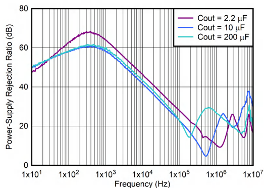
Figure 5-25. PSRR vs Frequency and C_{\text{OUT}}
