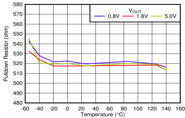
Figure 5-43. Smart Enable Pulldown Resistor vs Temperature and V_{OUT}
