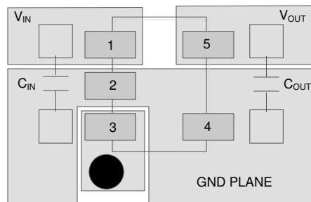
Figure 7-7. Layout Example for the DBV Package
