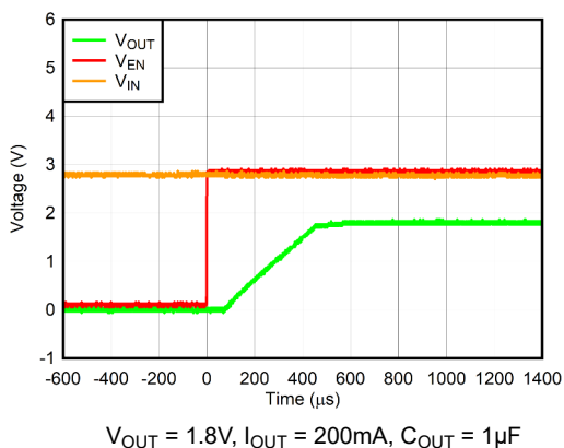
Figure 5-53. Start-Up With V_{EN} After V_{IN}
