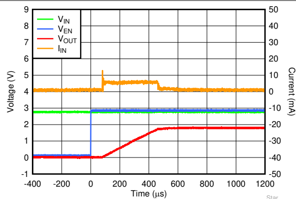
Figure 5-56. Start-Up Inrush Current With C_{OUT} = 1\mu\text{F}
