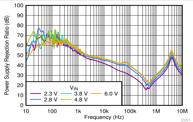
Figure 5-46. PSRR vs Frequency and V_{IN}
