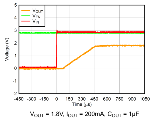
Figure 5-52. Start-Up With V_{EN} Before V_{IN}
