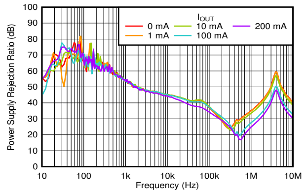
Figure 5-44. PSRR vs Frequency and I_{OUT}
