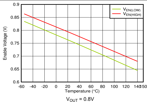
Figure 5-39. EN High and Low Threshold vs Temperature
