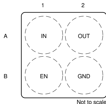
Figure 4-3. YCH Package, 4-Pin DSBGA, 0.35mm Pitch (Top View)
