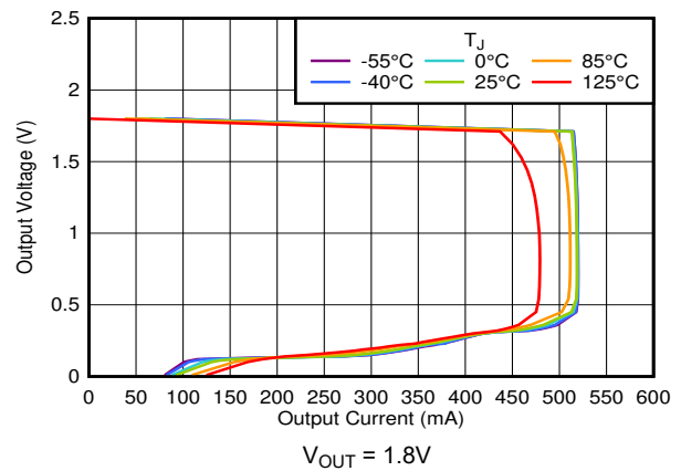
Figure 5-38. Foldback Current Limit vs I_{OUT} and Temperature
