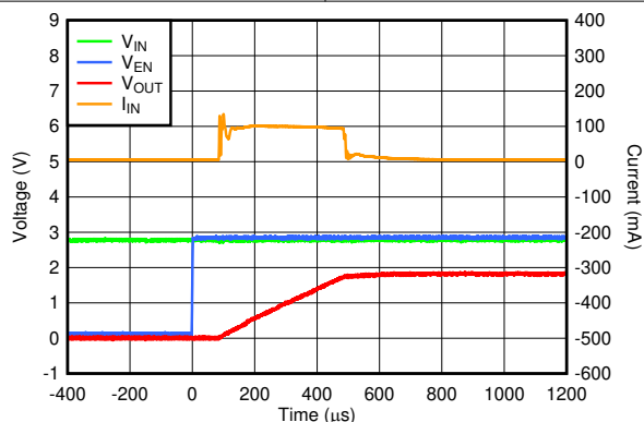
Figure 5-55. Start-Up With V_{EN} After V_{IN}
