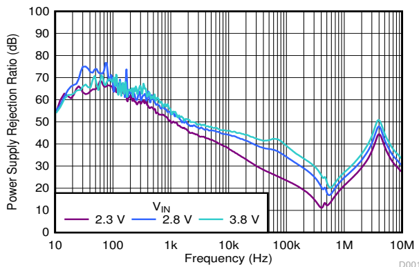
Figure 5-45. PSRR vs Frequency and V_{IN}
