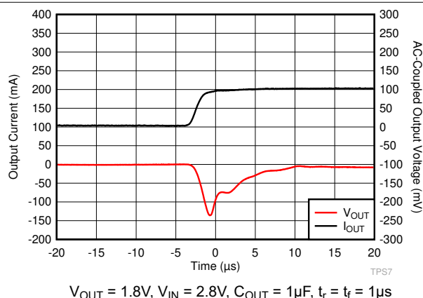
Figure 5-18. I_{OUT} Transient From 0mA to 100mA
