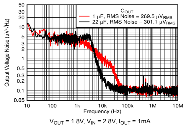
Figure 5-50. Output Noise vs Frequency and C_{OUT}
