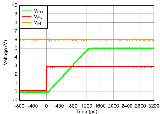
Figure 5-55. Start-Up With V_{EN} After V_{IN}
