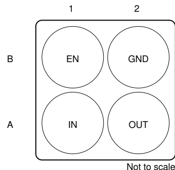
Figure 4-4. YCH Package, 4-Pin DSBGA, 0.35mm Pitch (Bottom View)
