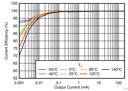
Figure 7-5. Current Efficiency vs I_{OUT} and Temperature
