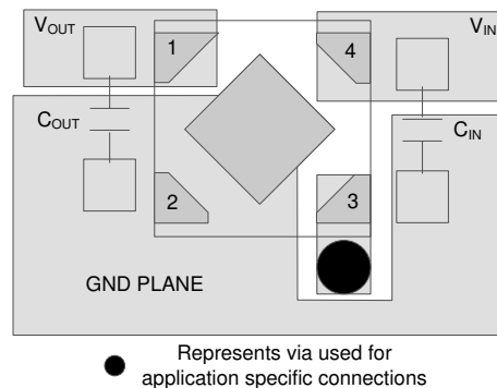
Figure 7-6. Layout Example for the DQN Package
