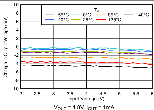
Figure 5-26. Line Regulation vs V_{IN} and Temperature
