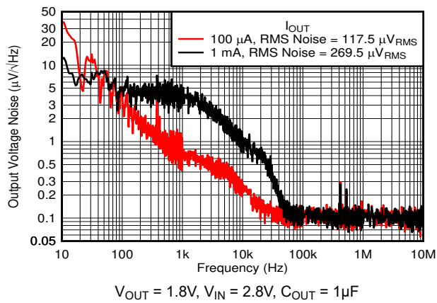
Figure 5-49. Output Noise vs Frequency and I_{OUT}
