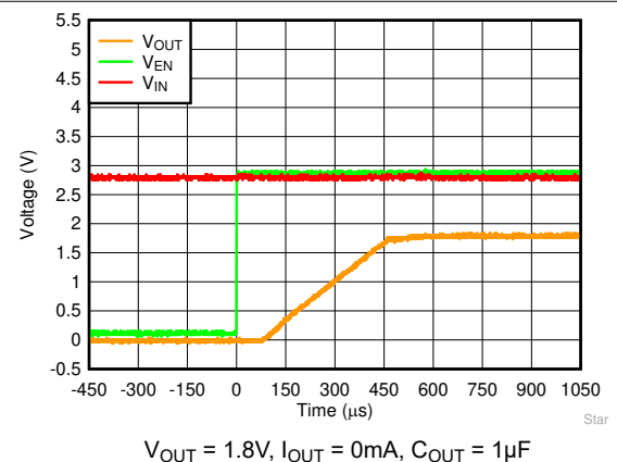
Figure 5-54. Start-Up With V_{EN} After V_{IN}
