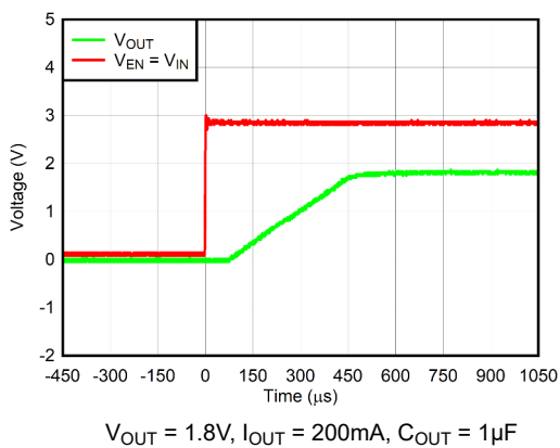
Figure 5-51. Start-Up With V_{EN} = V_{IN}
