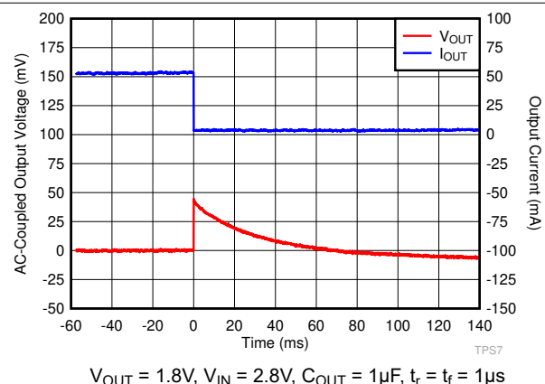
Figure 5-17. I_{OUT} Transient From 50mA to 0mA
