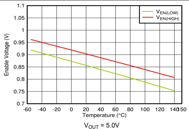
Figure 5-40. EN High and Low Threshold vs Temperature
