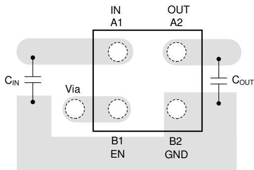
Figure 7-8. Layout Example for the YCH Package
