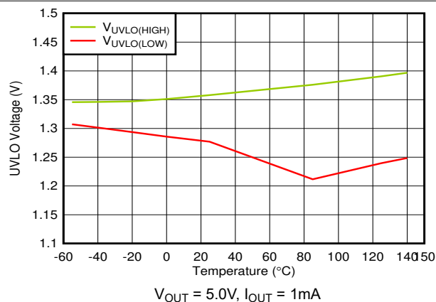
Figure 5-41. UVLO Rising and Falling Threshold vs Temperature
