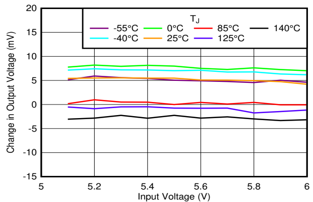
V_{OUT} = 5.0\text{ V} , I_{OUT} = 1\text{ mA} Figure 6-28. Line Regulation vs V_{IN} and Temperature
