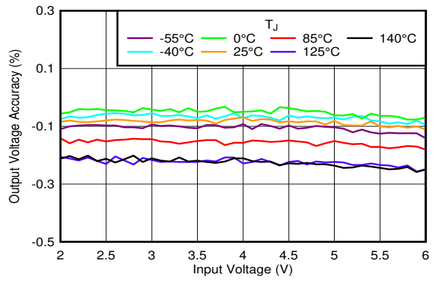
V_{OUT} = 1.8\text{ V} , I_{OUT} = 1\text{ mA} Figure 6-26. Output Accuracy vs V_{IN} and Temperature
