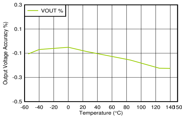
V_{OUT} = 1.8\text{ V} , I_{OUT} = 1\text{ mA} Figure 6-27. Output Accuracy vs Temperature
