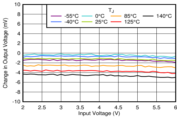
V_{OUT} = 1.8\text{ V} , I_{OUT} = 1\text{ mA} Figure 6-25. Line Regulation vs V_{IN} and Temperature
