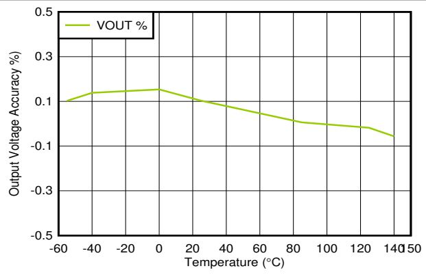
V_{OUT} = 5.0\text{ V} , I_{OUT} = 1\text{ mA} Figure 6-30. Output Accuracy vs Temperature
