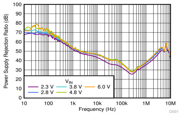
V_{OUT} = 1.8\text{ V} , I_{OUT} = 20\text{ mA} , C_{OUT} = 1\text{ }\mu\text{F} Figure 6-44. PSRR vs Frequency and V_{IN}
