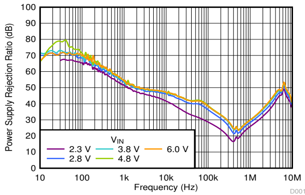
V_{OUT} = 1.8\text{ V} , I_{OUT} = 100\text{ mA} , C_{OUT} = 1\text{ }\mu\text{F} Figure 6-45. PSRR vs Frequency and V_{IN}
