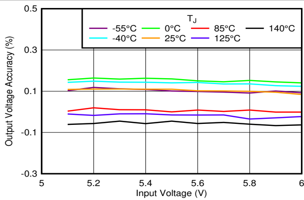
V_{OUT} = 5.0\text{ V} , I_{OUT} = 1\text{ mA} Figure 6-29. Output Accuracy vs V_{IN} and Temperature
