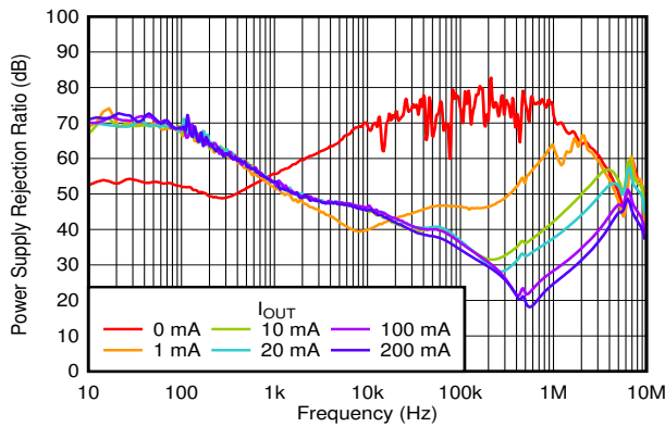
V_{IN} = 2.8\text{ V} , V_{OUT} = 1.8\text{ V} , C_{OUT} = 1\text{ }\mu\text{F} Figure 6-43. PSRR vs Frequency and I_{OUT}
