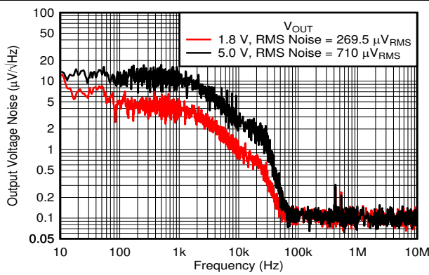
V_{IN} = V_{OUT} + 1.0\text{ V} , I_{OUT} = 1\text{ mA} , C_{OUT} = 1\text{ }\mu\text{F} Figure 6-47. Output Noise vs Frequency and V_{OUT}
