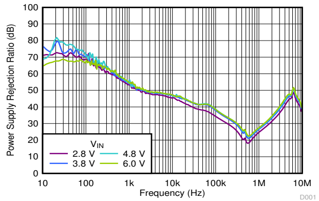
V_{OUT} = 1.8\text{ V} , I_{OUT} = 200\text{ mA} , C_{OUT} = 1\text{ }\mu\text{F} Figure 6-46. PSRR vs Frequency and V_{IN}
