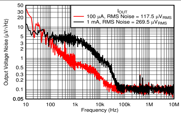
V_{OUT} = 1.8\text{ V} , V_{IN} = 2.8\text{ V} , C_{OUT} = 1\text{ }\mu\text{F} Figure 6-48. Output Noise vs Frequency and I_{OUT}
