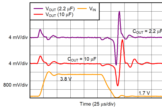
Figure 5-32. V_{IN} Line Transient (new chip)
