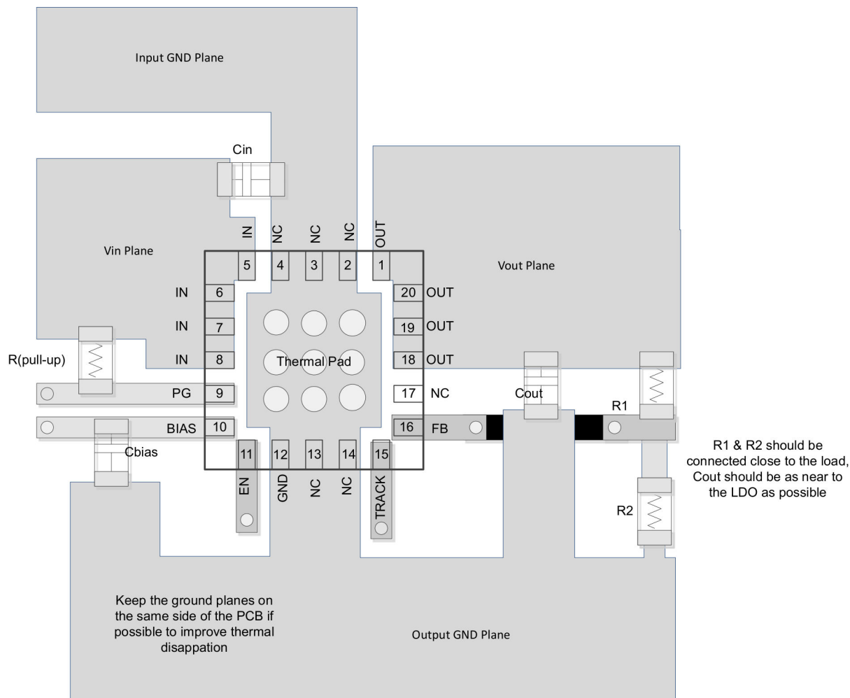
Figure 7-10. Layout Example
