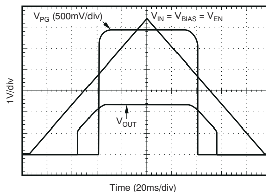
Figure 5-36. Power-Up/Power-Down (legacy chip)
