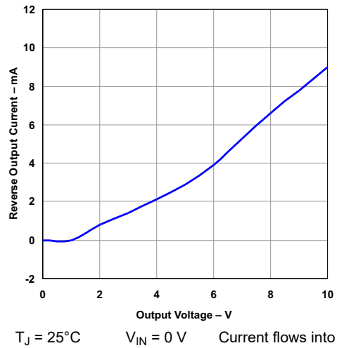
Figure 5-16. Reverse Output Current vs Output Voltage
