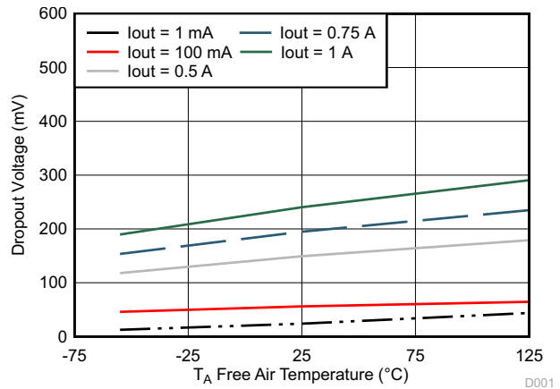
Figure 5-2. Dropout Voltage vs Temperature
