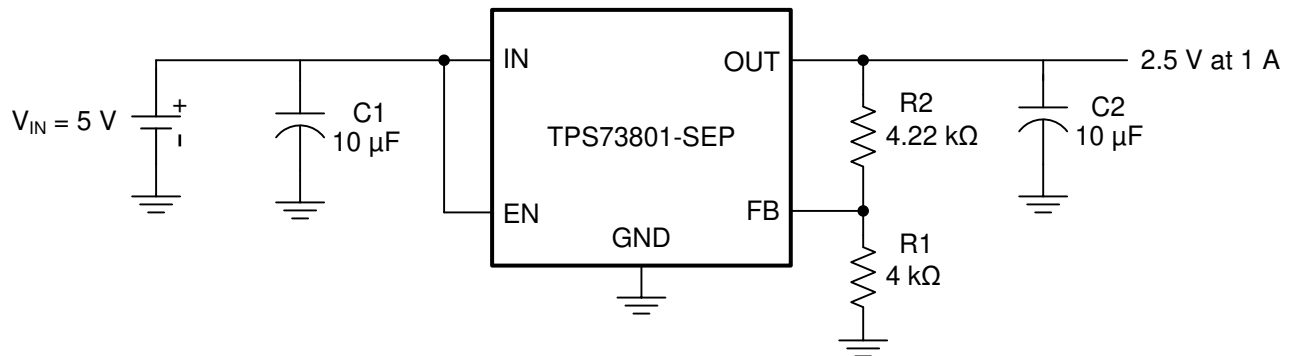
Figure 7-1. Adjustable Output Voltage Operation
