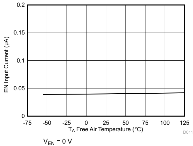
Figure 5-9. EN Input Current vs Temperature
