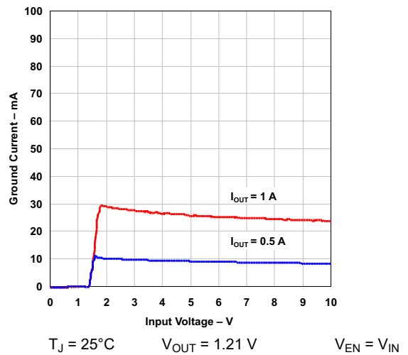
Figure 5-6. Ground Current vs Input Voltage
