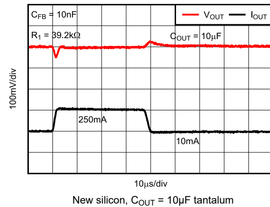
Figure 5-50. TPS73701 Load Transient, Adjustable Version
