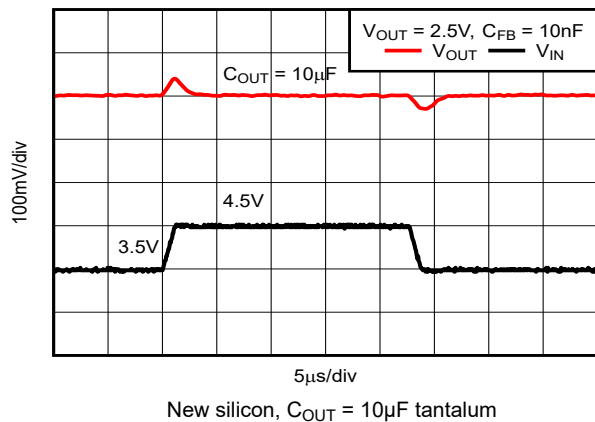
Figure 5-52. TPS73701 Line Transient, Adjustable Version
