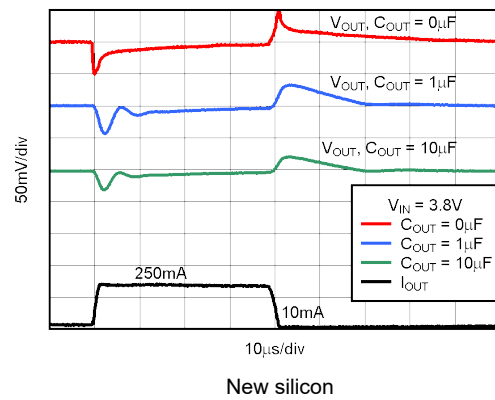
Figure 7-6. TPS73233 Load Transient Response
