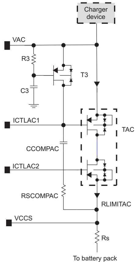
Figure 5-55. Typical Application Schematic (In-Rush Current Limitation)
