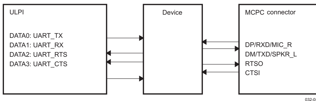
Figure 5-49. MCPC UART and Handshake Mode Data Flow
