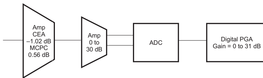
Figure 5-40. Carkit Input Uplink Path Characteristics
