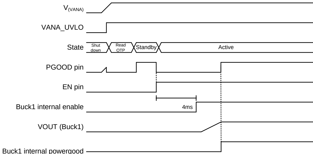
Figure 13. PGOOD Pin Operation in Continuous Mode
