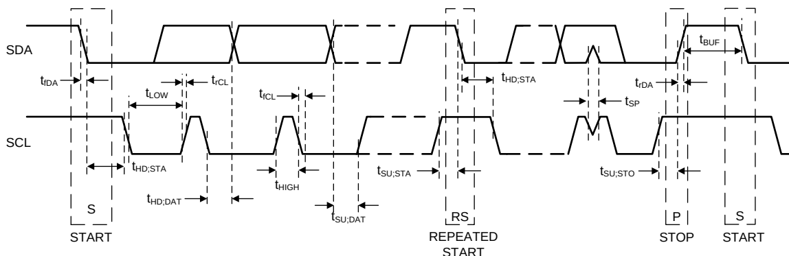
Figure 18. I²C-Compatible Timing
