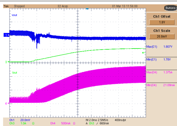
Figure 8-34. Buck 2 PFM to PWM Transition Ch1 = V_{OUT} Ch3 = I_{OUT} Ch4 = Inductor
