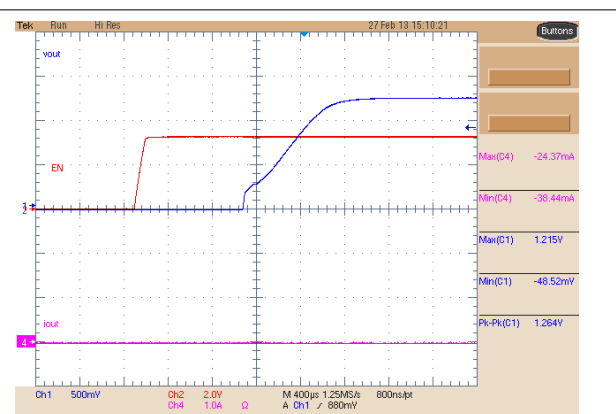
Figure 8-4. Buck 1 Soft-Start
