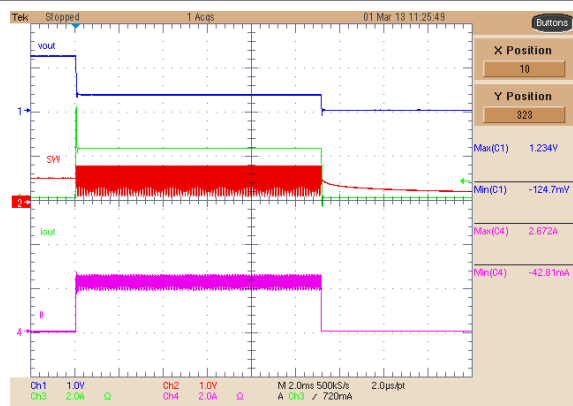
Figure 8-18. Buck 1 Current Limit Operation, Hiccup
