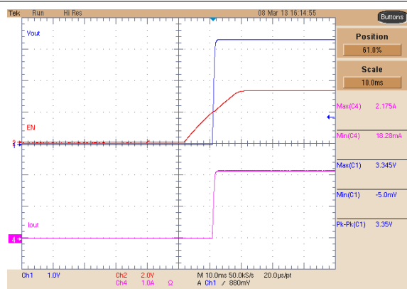
Figure 8-38. Buck 3 Soft-Start
