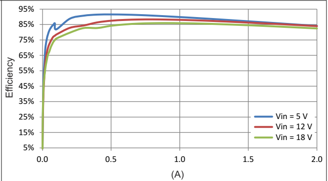
Figure 6-8. Efficiency, LOW_P Mode
