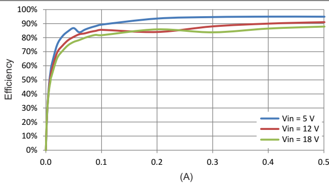
Figure 6-13. Efficiency, Forced PWM
