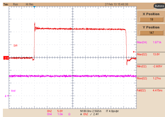
Figure 8-41. Buck 3 Switching Node, 1.5-A Load
