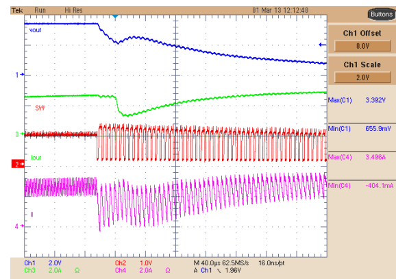
Figure 8-48. Buck 3 PFM to PWM Transition
