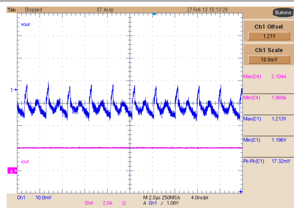
Figure 8-15. Buck 1 Ripple, 2-A Load
