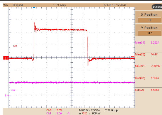
Figure 8-27. Buck 2 Switching Node, 2-A Load
