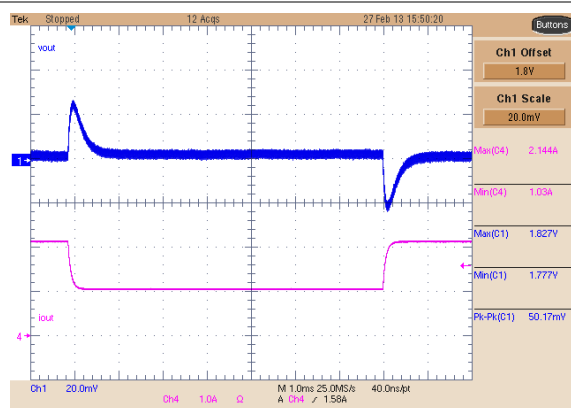
Figure 8-29. Buck 2 Dynamic Response, 1-A to 2-A Step
