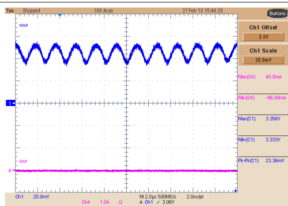
Figure 8-44. Buck 3 Ripple, No Load
