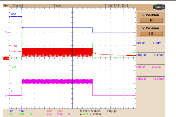
Figure 8-18. Buck 1 Current Limit Operation, Hiccup
