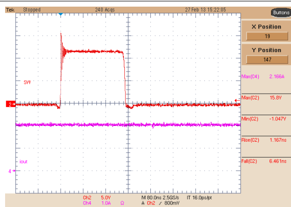
Figure 8-9. Buck 1 Switching Node, 2-A Load
