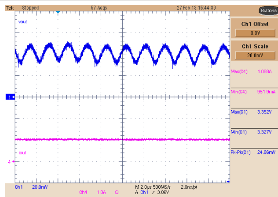
Figure 8-45. Buck 3 Ripple, 1-A Load
