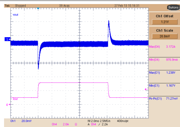
Figure 8-13. Buck 1 Dynamic Response, 1-A to 3-A Step
