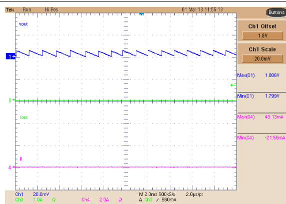
Figure 8-33. Buck 2 Low-Power Output, No Load
