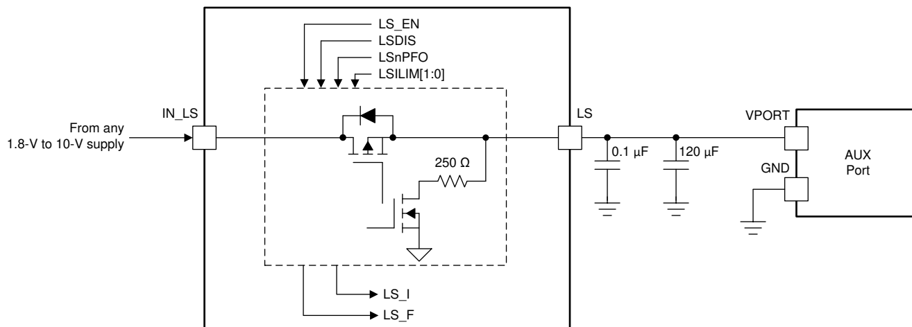
Figure 6-10. Typical Application of Load Switch
