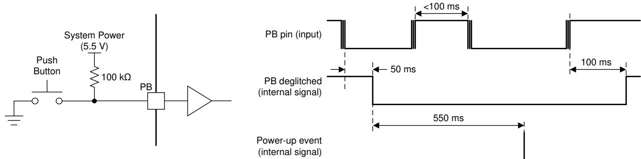
Figure 6-15. Left: Typical PB Input Circuit Right: Push-Button Input (PB) Deglitch and Power-Up Timing
