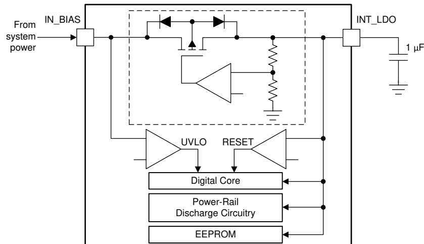
Figure 6-9. Internal LDO and UVLO Sensing
