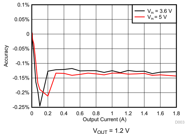
Figure 5-3. DCDC3 Accuracy
