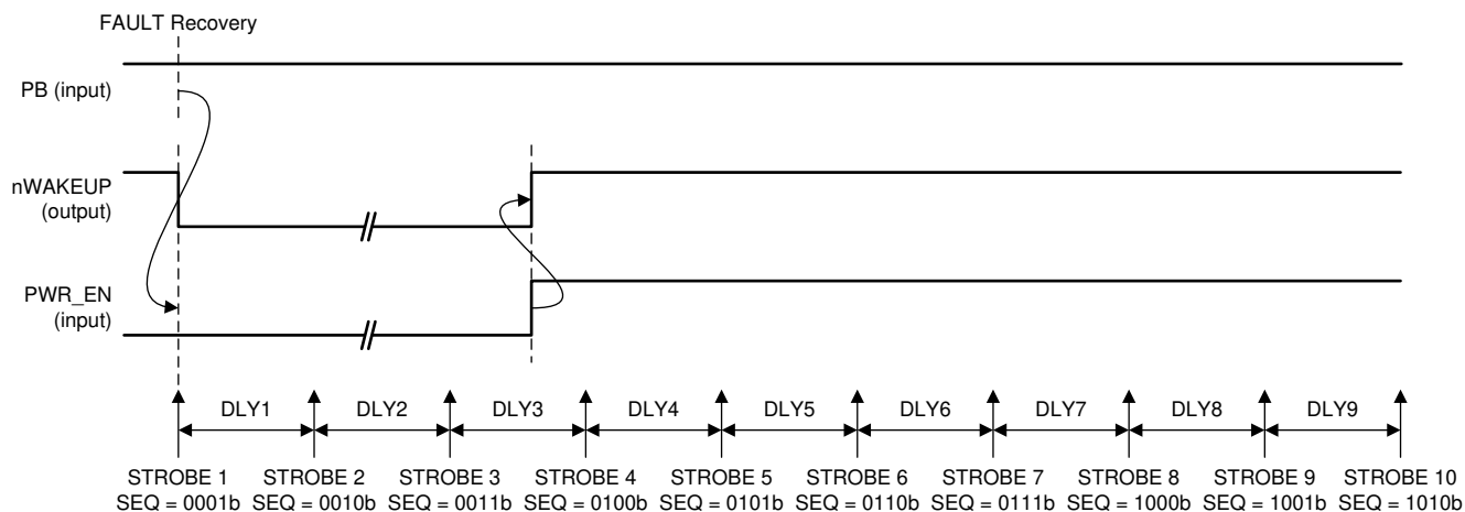
Figure 6-3. Power-Up Sequences from RECOVERY State
