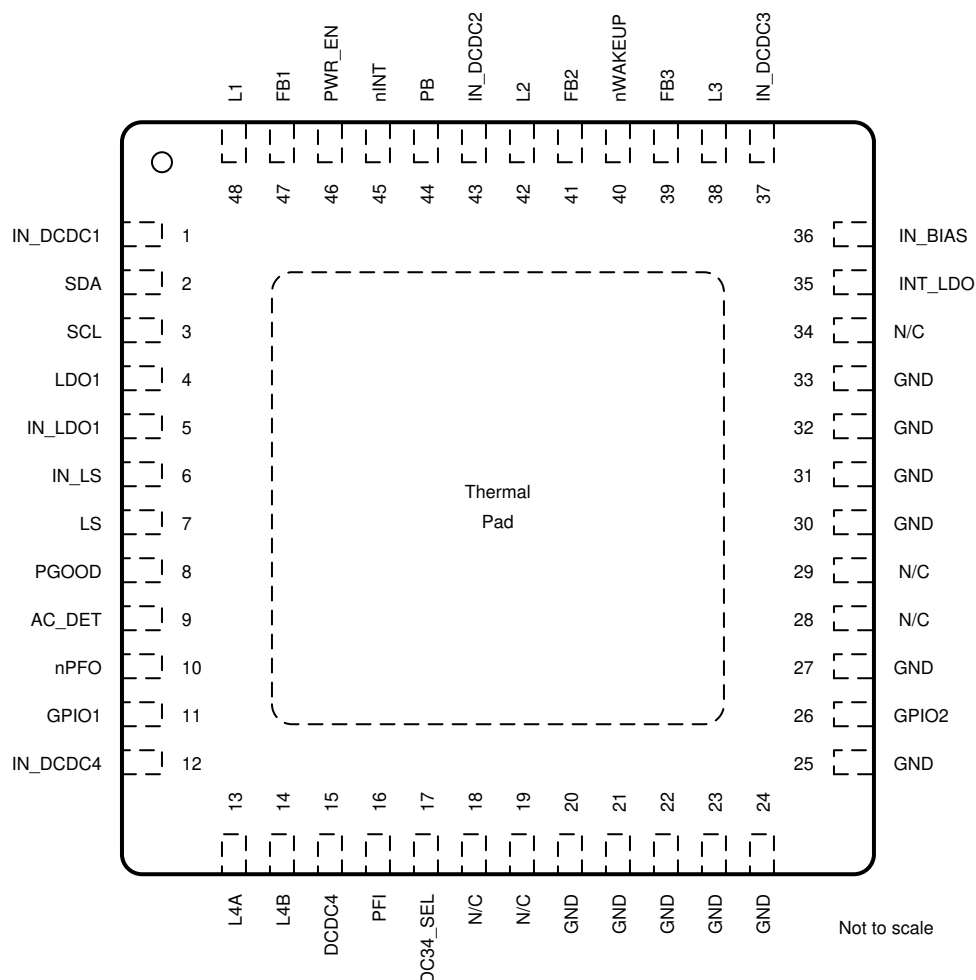
Figure 4-1. 48-Pin RSL VQFN With Exposed Thermal Pad (Top View, 6 mm × 6 mm × 1 mm With 0.4-mm Pitch)
