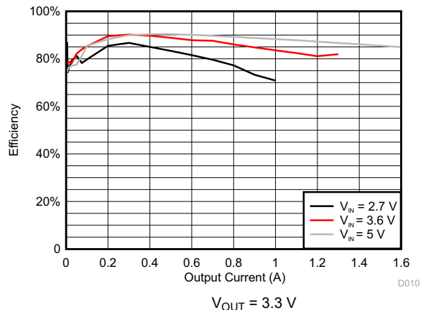
Figure 8-5. DCDC4 Efficiency
