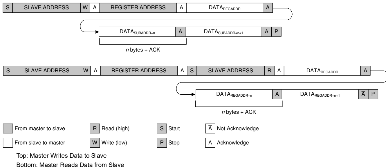
Figure 6-21. I 2 C Data Protocol
