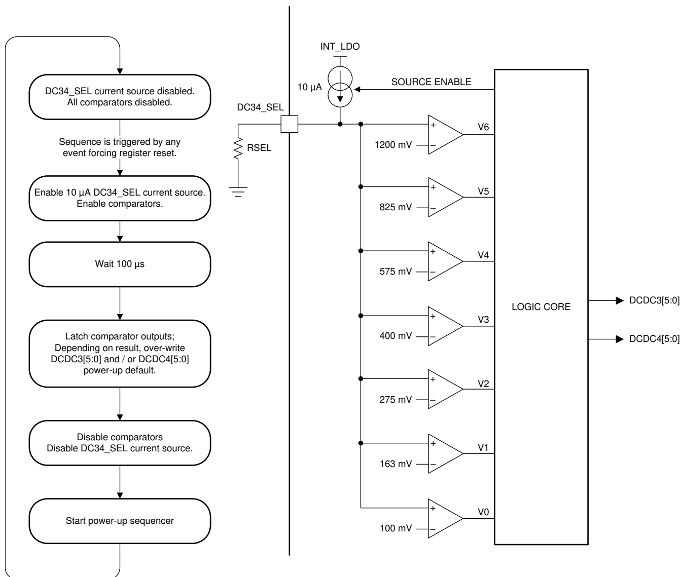
Figure 6-13. Left: Flow Chart for Selecting DCDC Power-Up Default Voltage Right: Comparator Circuit
