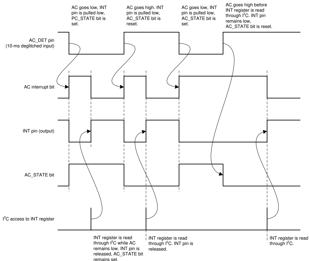
Figure 6-19. AC_STATE Pin
