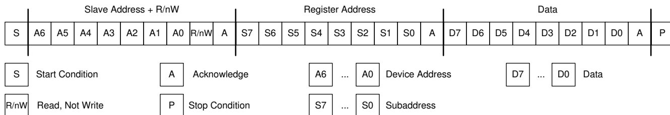
Figure 6-20. Subaddress in I 2 C Transmission
