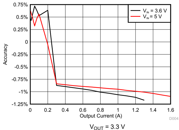
Figure 5-4. DCDC4 Accuracy
