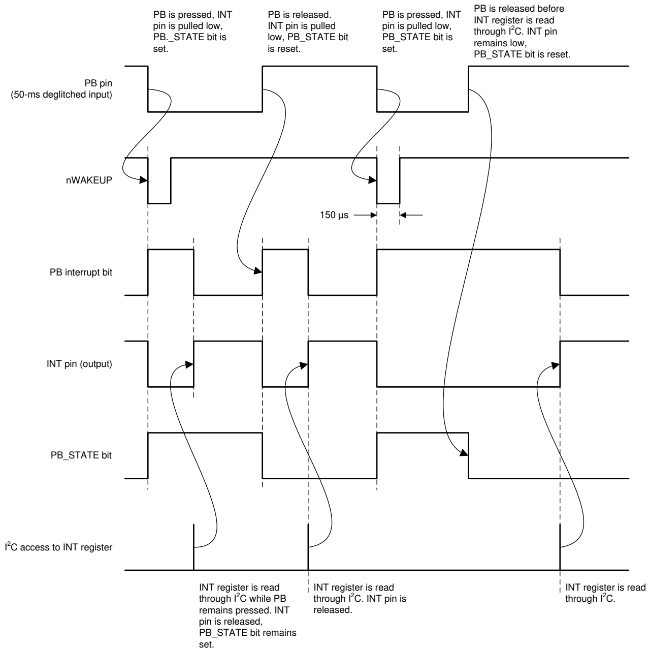
Figure 6-16. PB Input-Low or Input-High Thresholds
