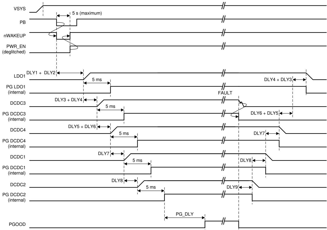
Figure 6-8. Typical Power-Up Sequence of the Main Output Rails
