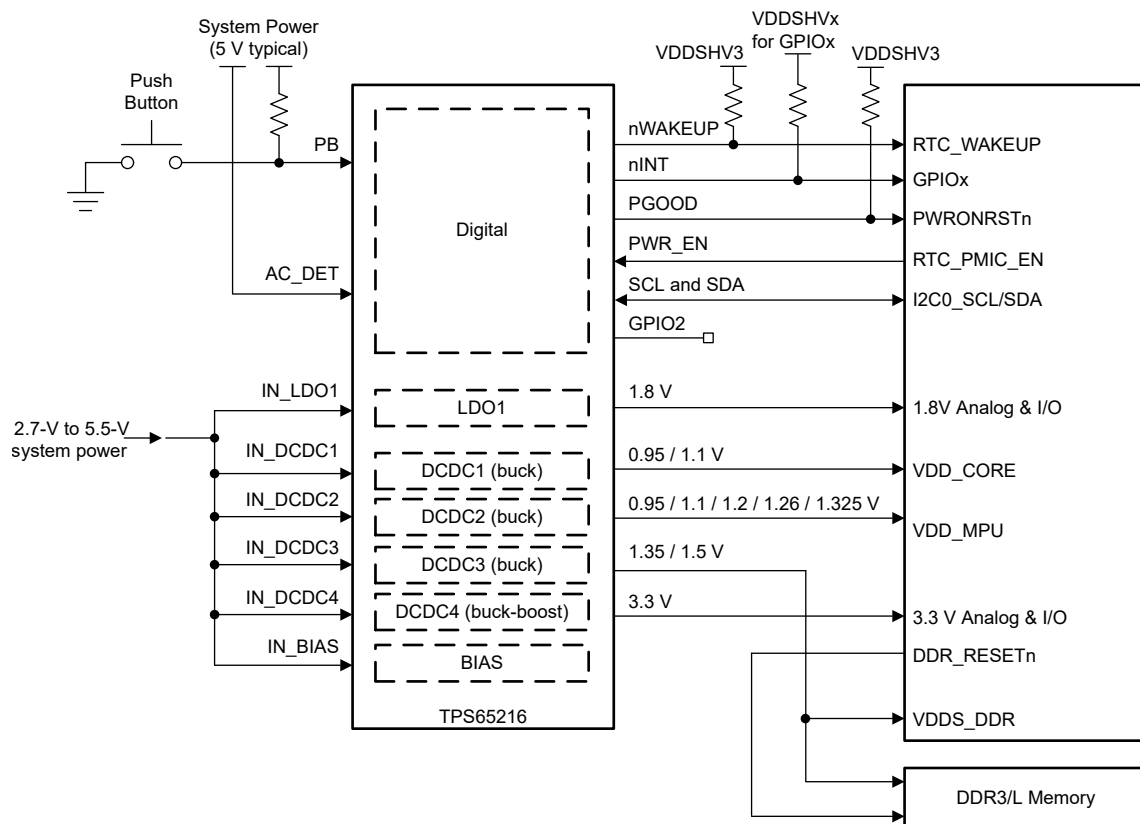
Figure 8-1. Typical Application Schematic
