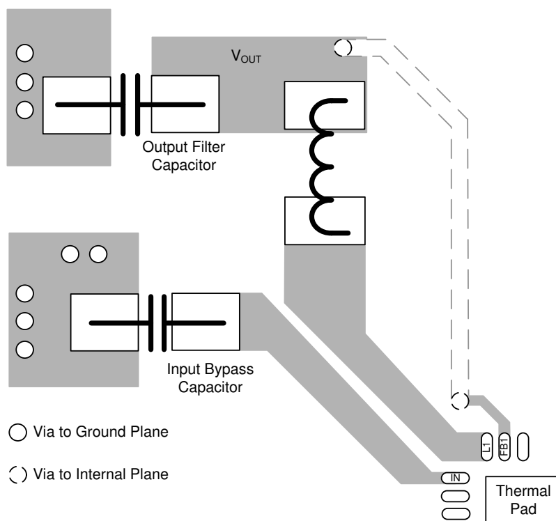
Figure 8-6. Layout Recommendation
