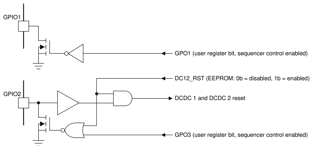
Figure 6-14. I/O Pin Logic
