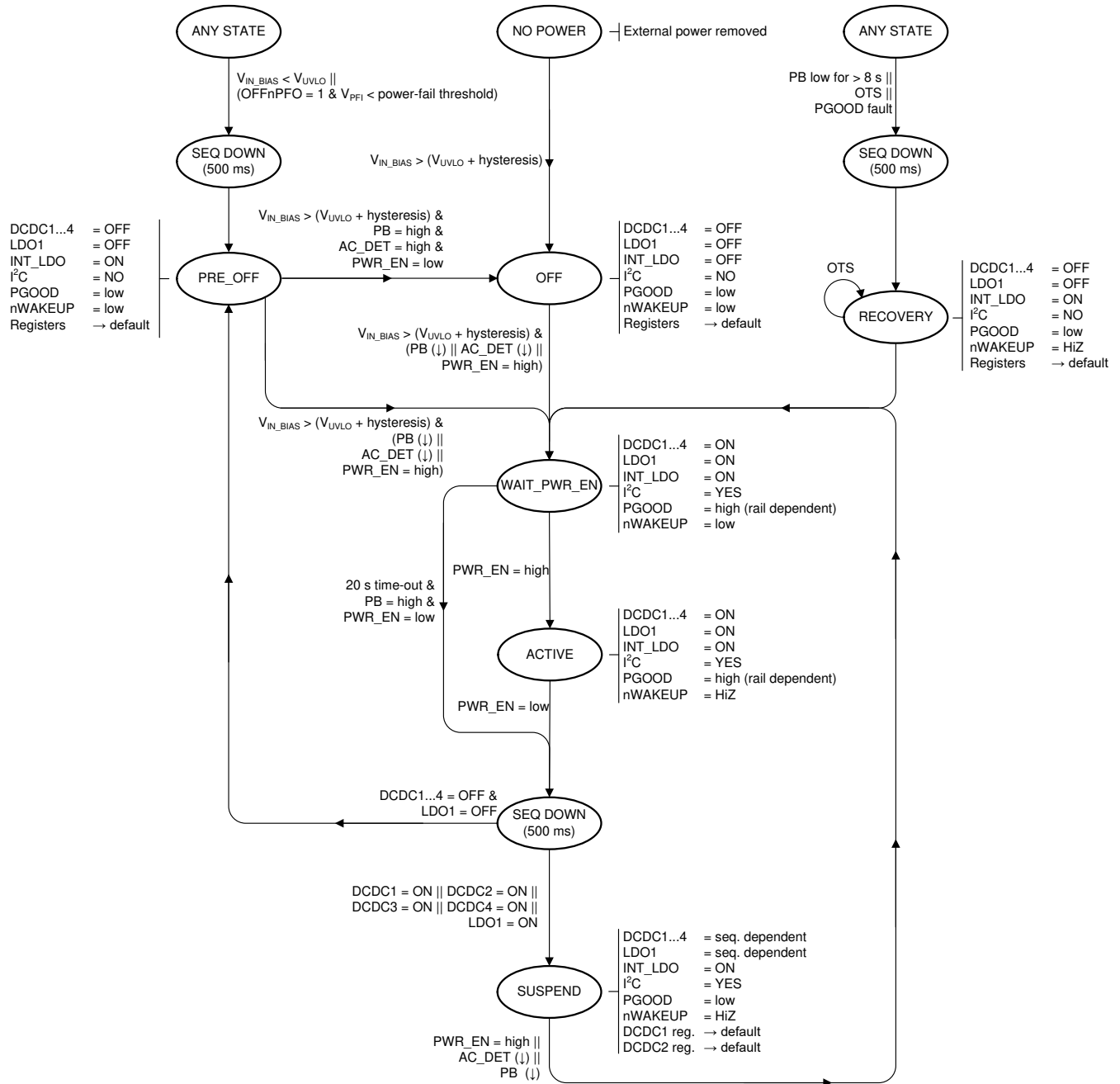
Figure 6-24. Modes of Operation Diagram
