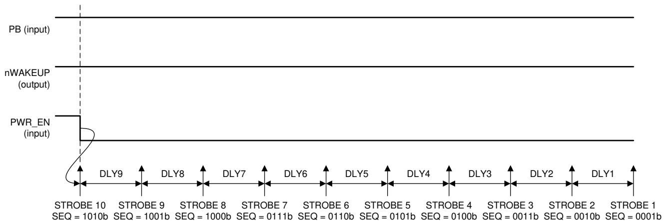
Figure 6-4. Power-Down Sequences to OFF State; PWR_EN is Power-Down Event
