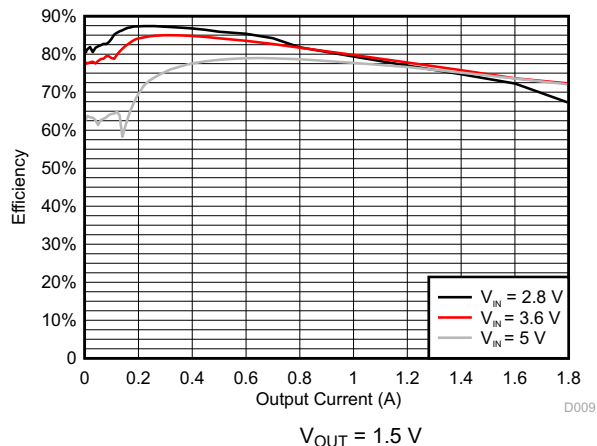
Figure 8-4. DCDC3 Efficiency
