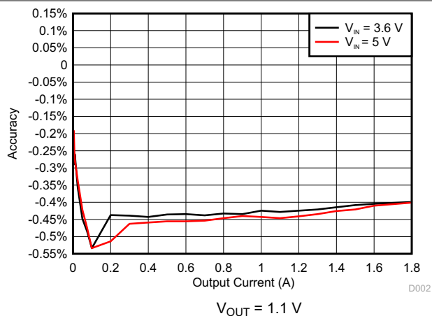
Figure 5-2. DCDC2 Accuracy
