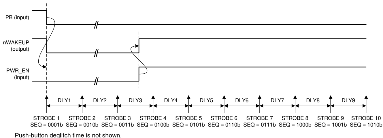
Figure 6-1. Power-Up Sequences from OFF or SUSPEND State; PB is Power-Up Event
