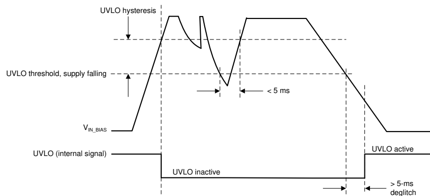
Figure 6-11. Definition of UVLO and Hysteresis
