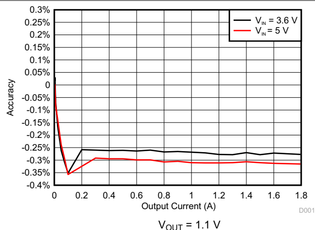
Figure 5-1. DCDC1 Accuracy
