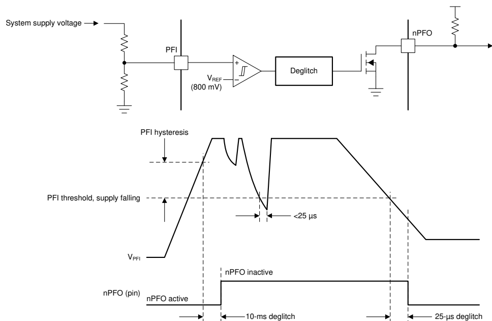
Figure 6-12. Power-Fail Comparator Simplified Circuit and Timing Diagram
