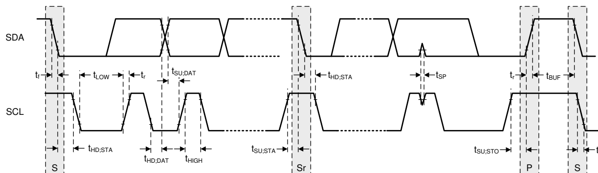
Figure 6-23. I²C Protocol and Transmission Timing I²C Data Transmission Timing
