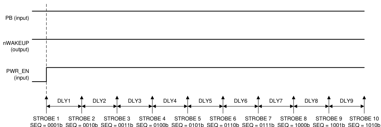
Figure 6-2. Power-Up Sequences from SUSPEND State; PWR_EN is Power-Up Event
