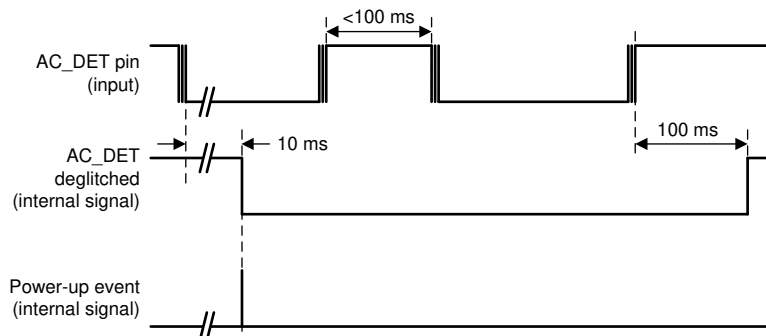
Figure 6-18. AC_DET Input Deglitch and Power-Up Timing (Portable Systems)
