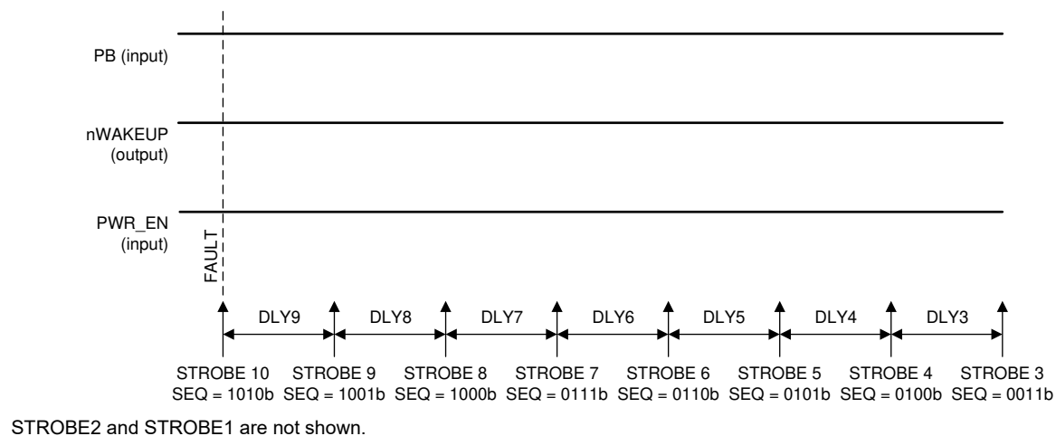
Figure 6-6. Power-Down Sequences to RECOVERY State; TSD or UV is Power-Down Event
