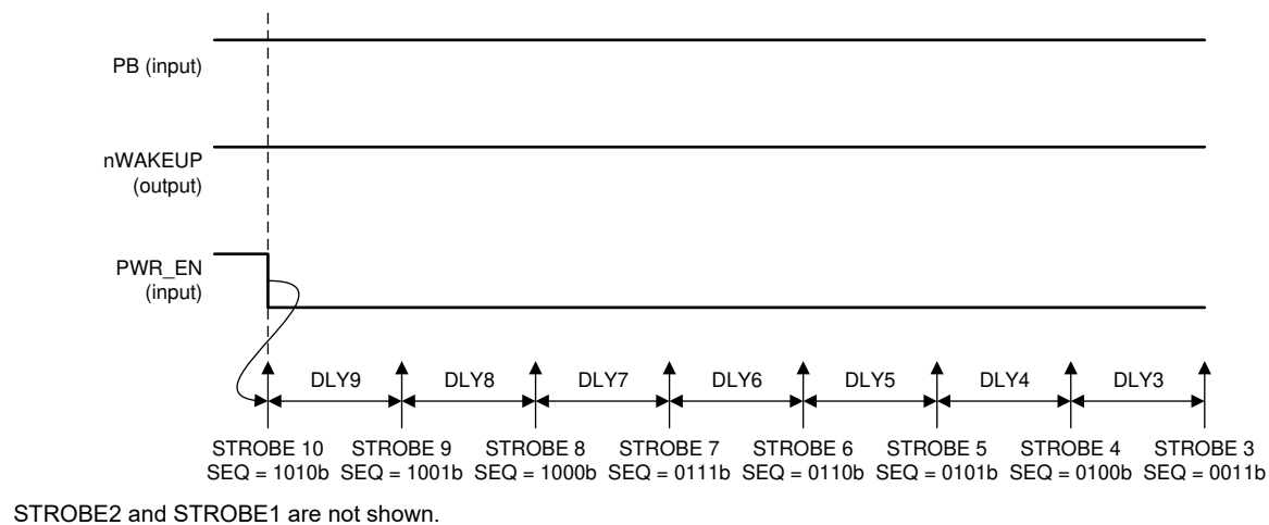
Figure 6-5. Power-Down Sequences to SUSPEND State; PWR_EN is Power-Down Event
