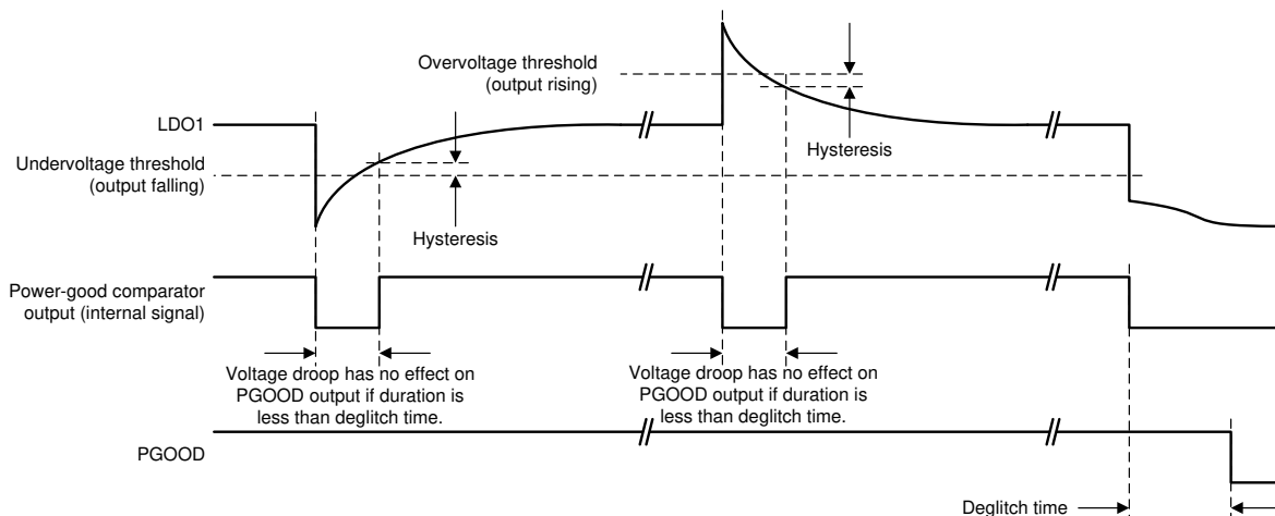
Figure 6-7. Definition of Undervoltage, Overvoltage Thresholds, Hysteresis, and Deglitch Times
